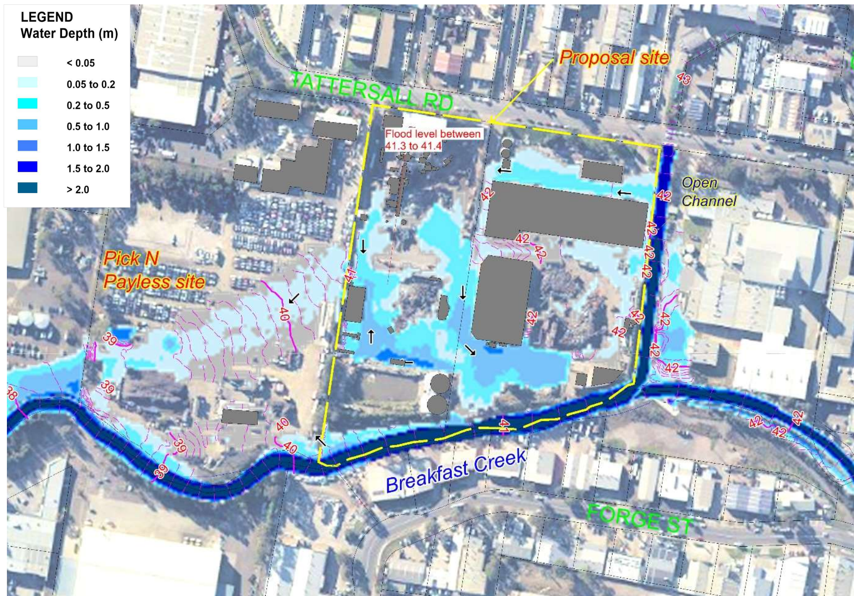
Figure 7 – 1% AEP Flood Depths and Levels
