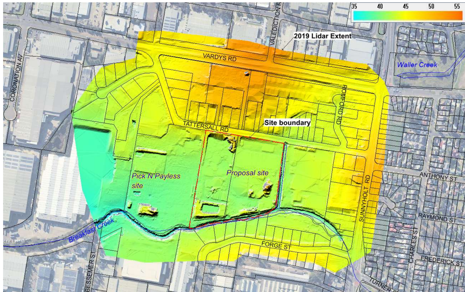
Figure 5 – Extent of 2019 Lidar Adopted in Flood Model
