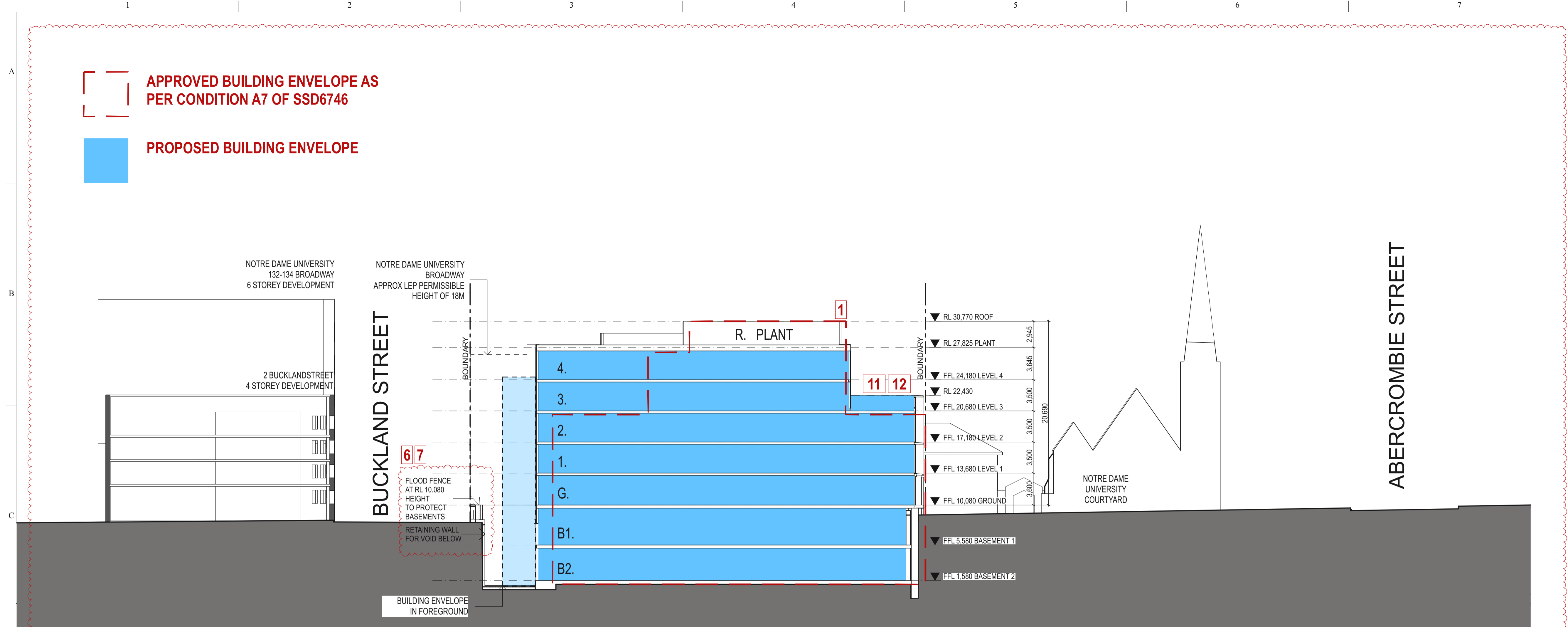
PROPOSED ENVELOPE SECTION-LOOKING NORTH 1:250 @A1
