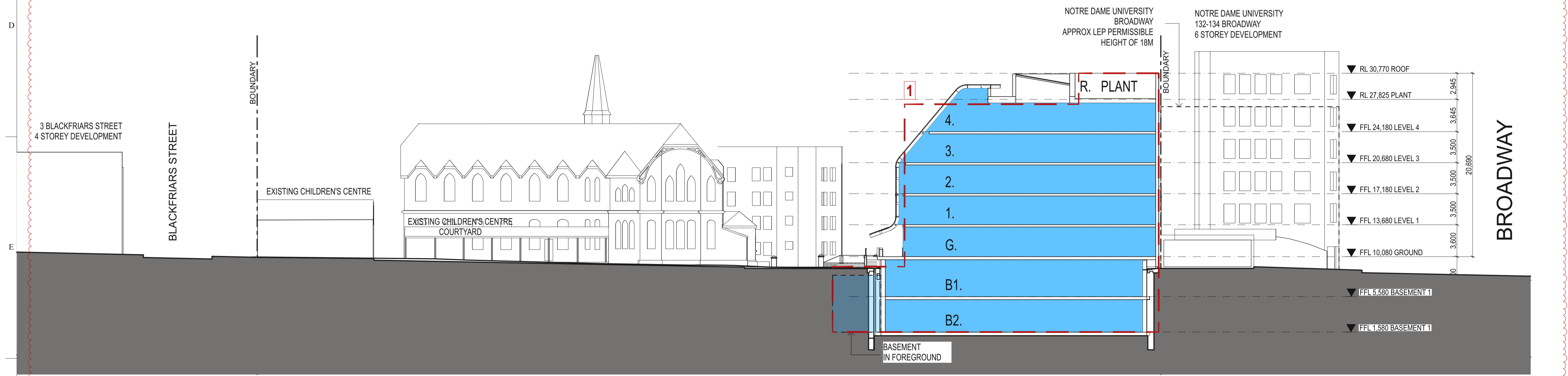
PROPOSED ENVELOPE SECTION-LOOKING WEST 1:250 @A1
