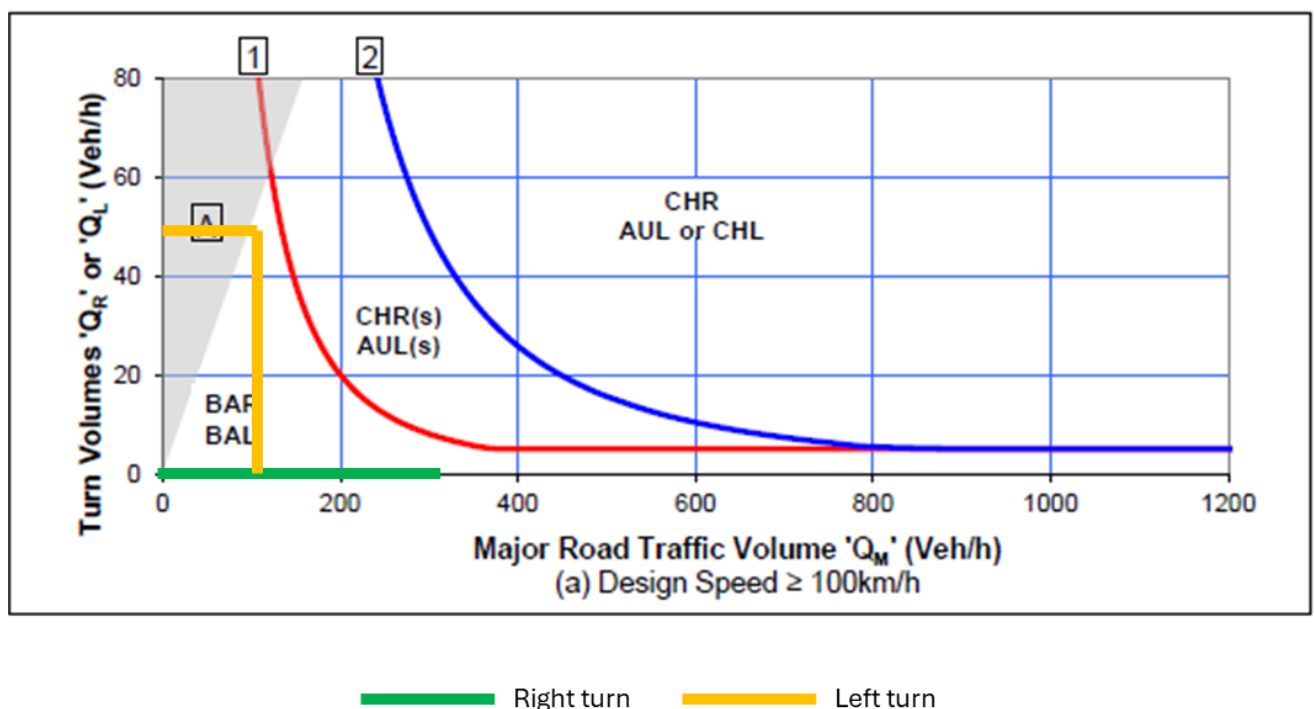
Figure 4.13 Access Point 2 / Castlereagh Highway intersection
