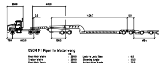
VEHICLE PROFILES (NOT TO SCALE)
