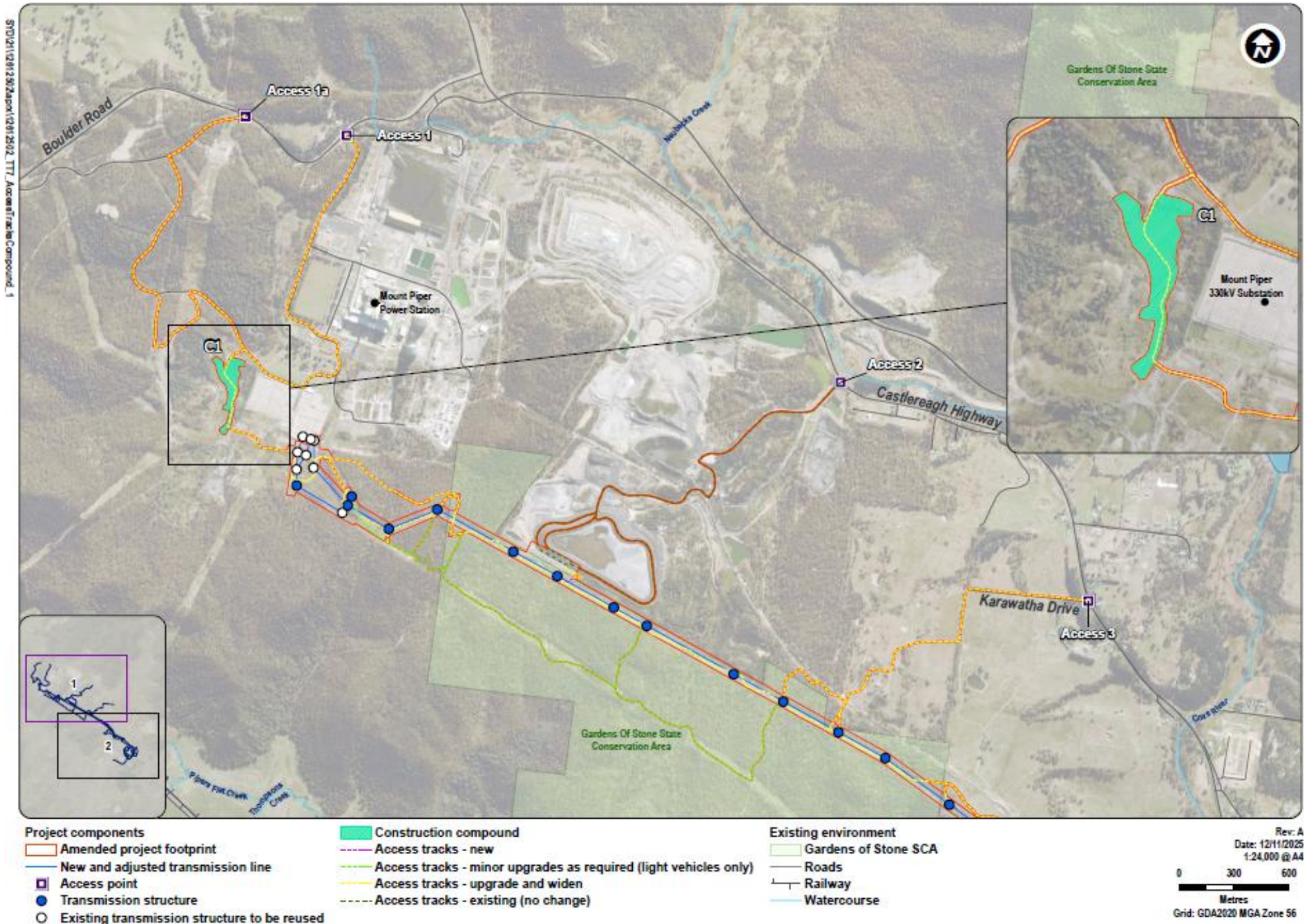
Figure 4.1 Construction access points 1 to 3
