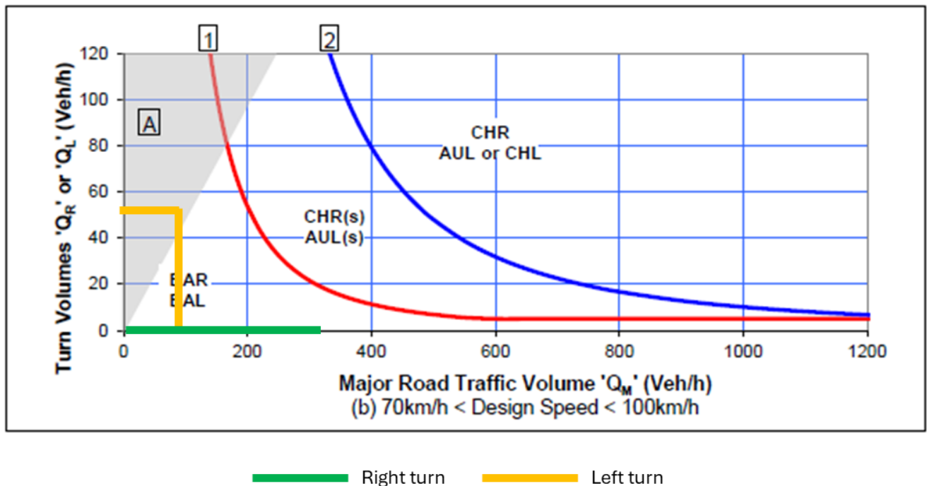
Figure 4.21 Access Point 10 / Castlereagh Highway
