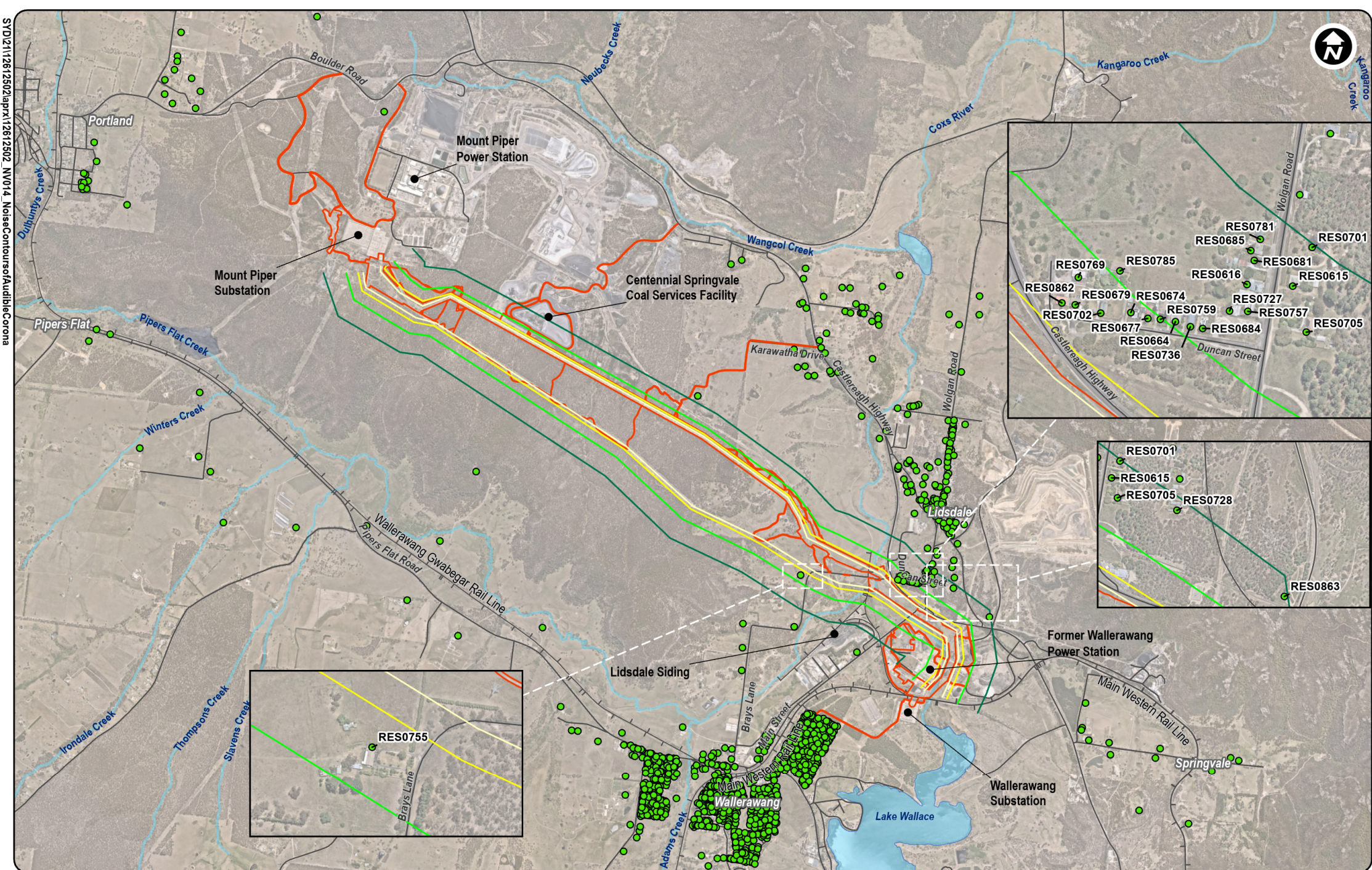
Figure 5.4 Updated Figure 6.11 from EIS – Noise contours of audible corona noise in L50 conditions 0 500 1,000 Metres Grid: GDA2020 MGA Zone 56
