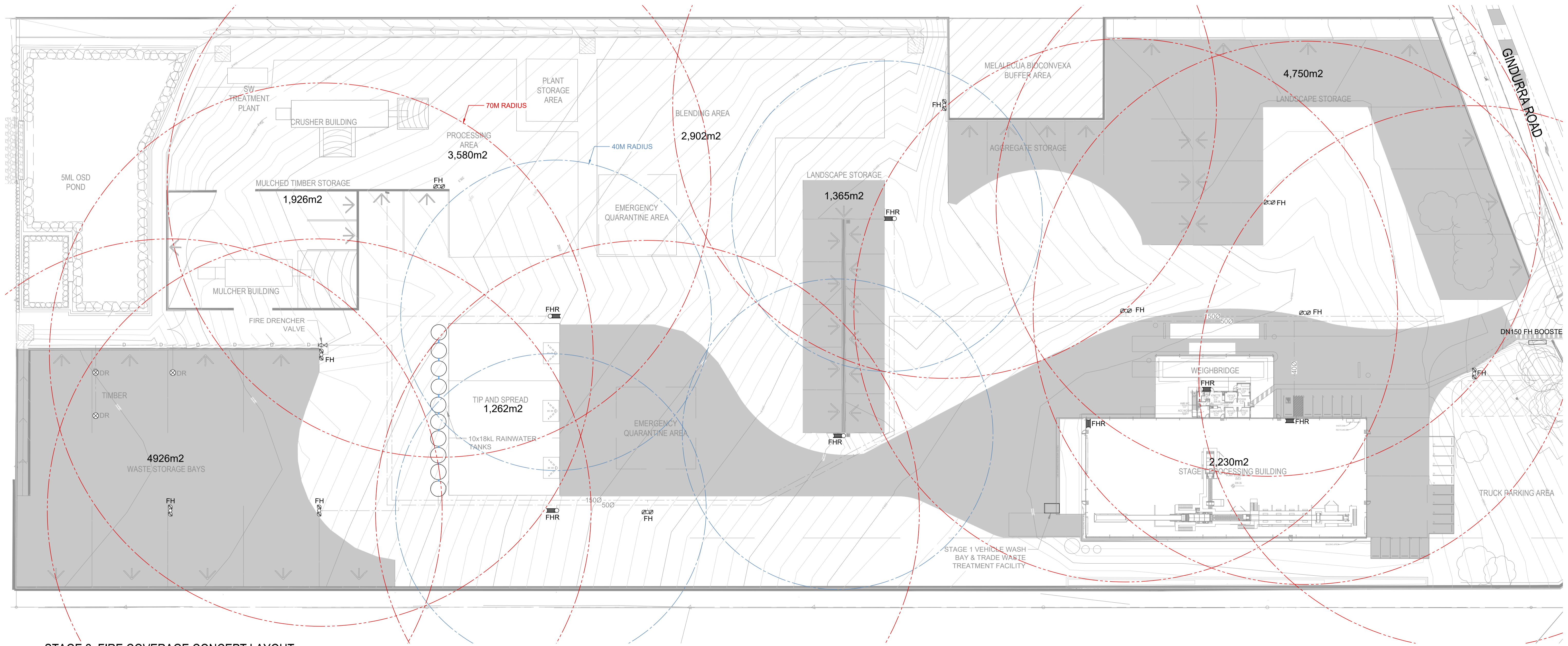
STAGE 2 FIRE COVERAGE CONCEPT LAYOUT SCALE 1:500
