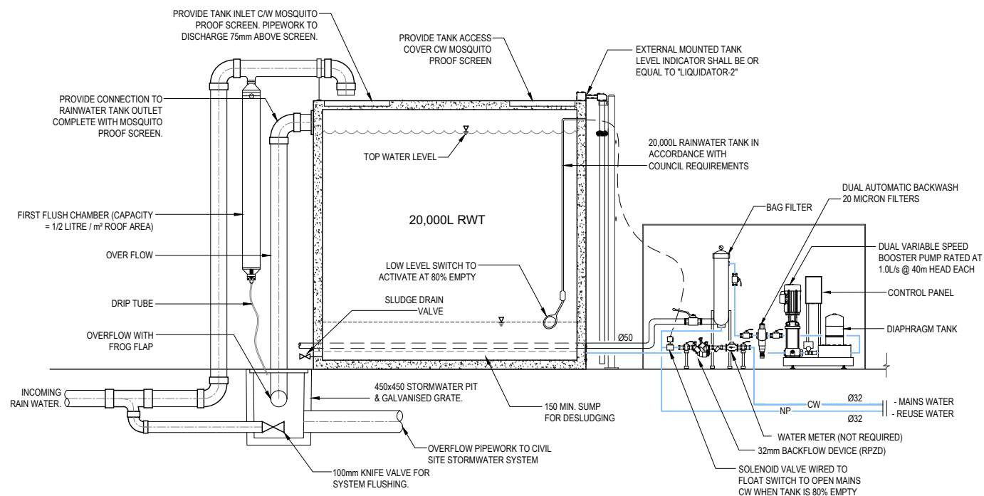
D02 H101 RAINWATER RE-USE TANK DETAIL (GUIDE ONLY) N.T.S.
