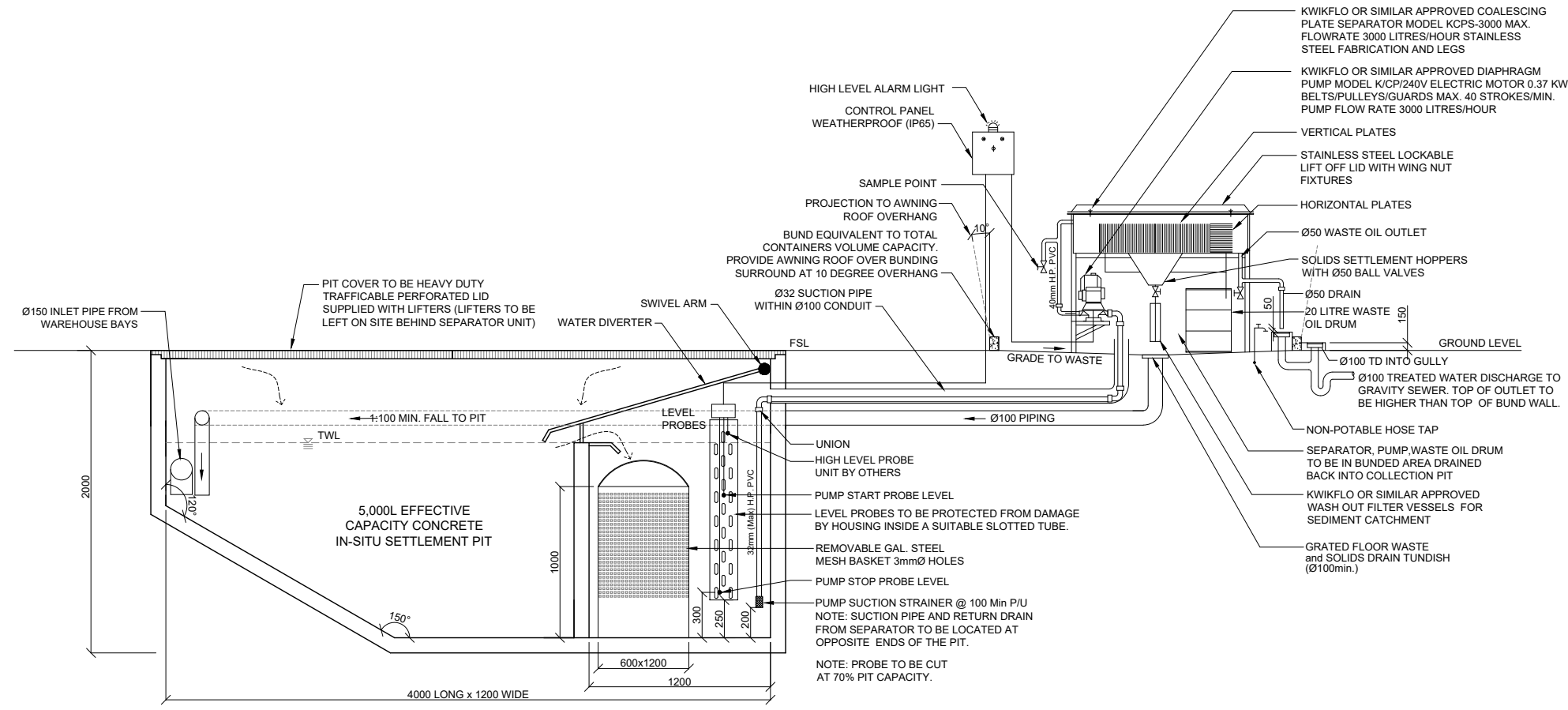
D01 H101 WASH DOWN BAY / OIL ARRESTOR N.T.S. STEP IRONS AND PLATFORMS ARE TO BE INSTALLED AS REQUIRED
