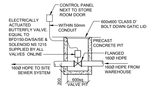
D03 H101 TYPICAL VALVE PIT DETAIL N.T.S.
