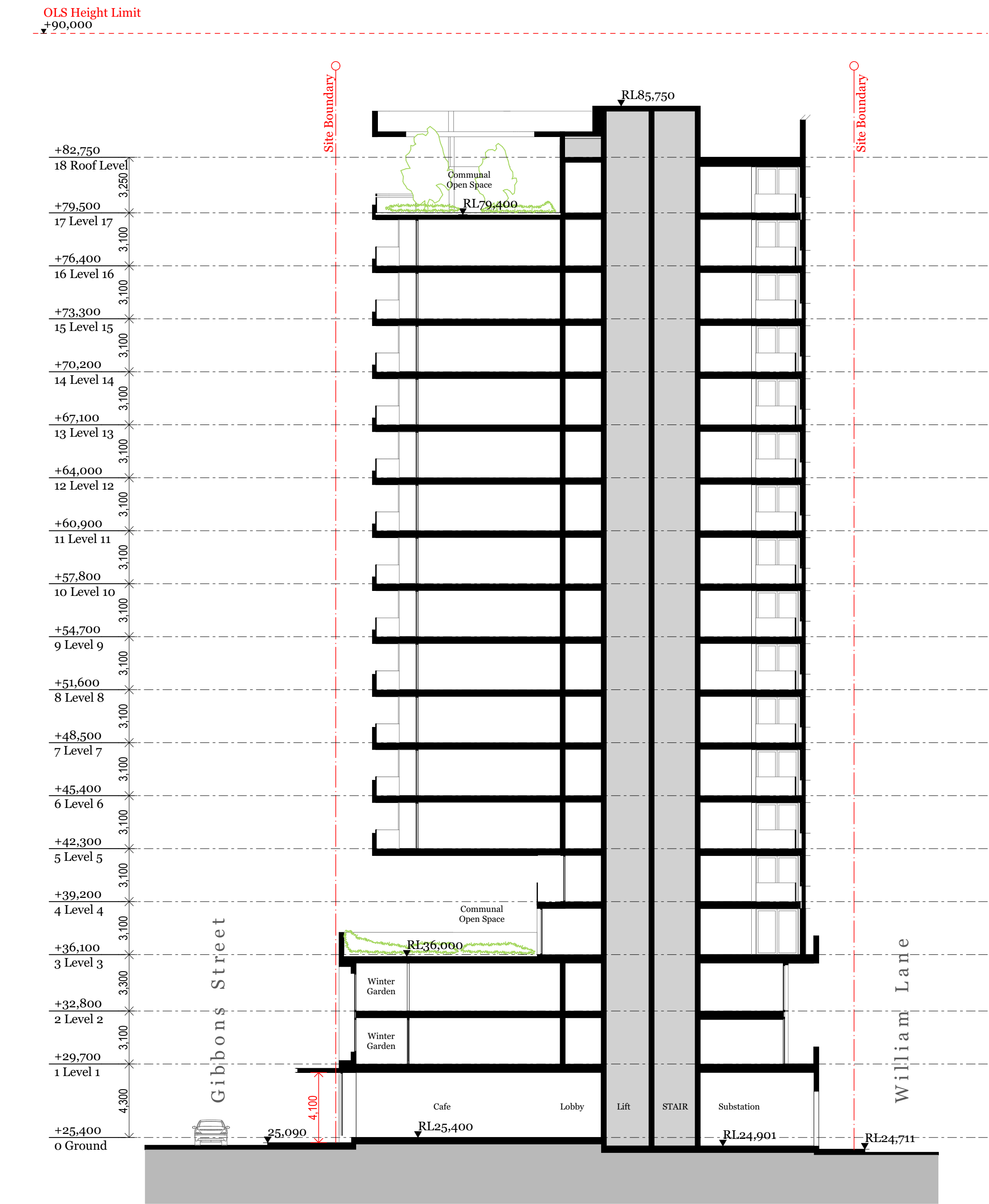
S03 Section 3 1:200
