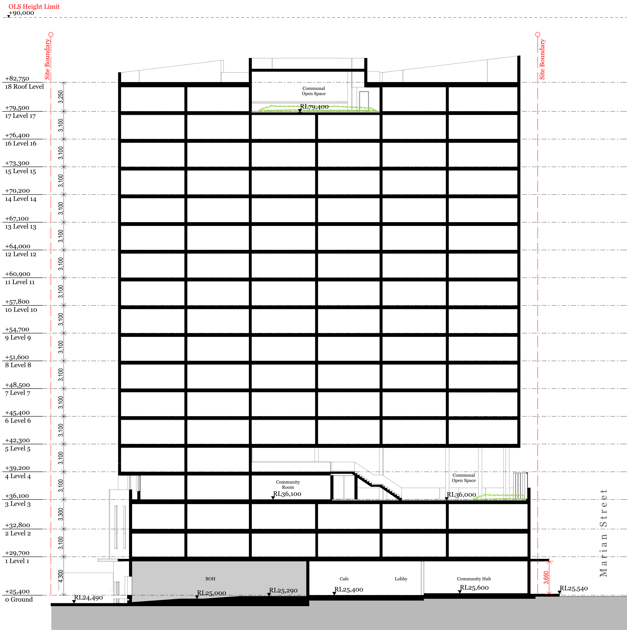
S04 Section 4 1:200
