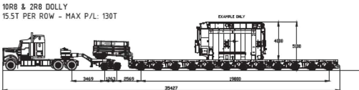
Figure 4 - The largest vehicle anticipated to access the site (source: OSOM Route Study, Ares Group, Jan 2026)
