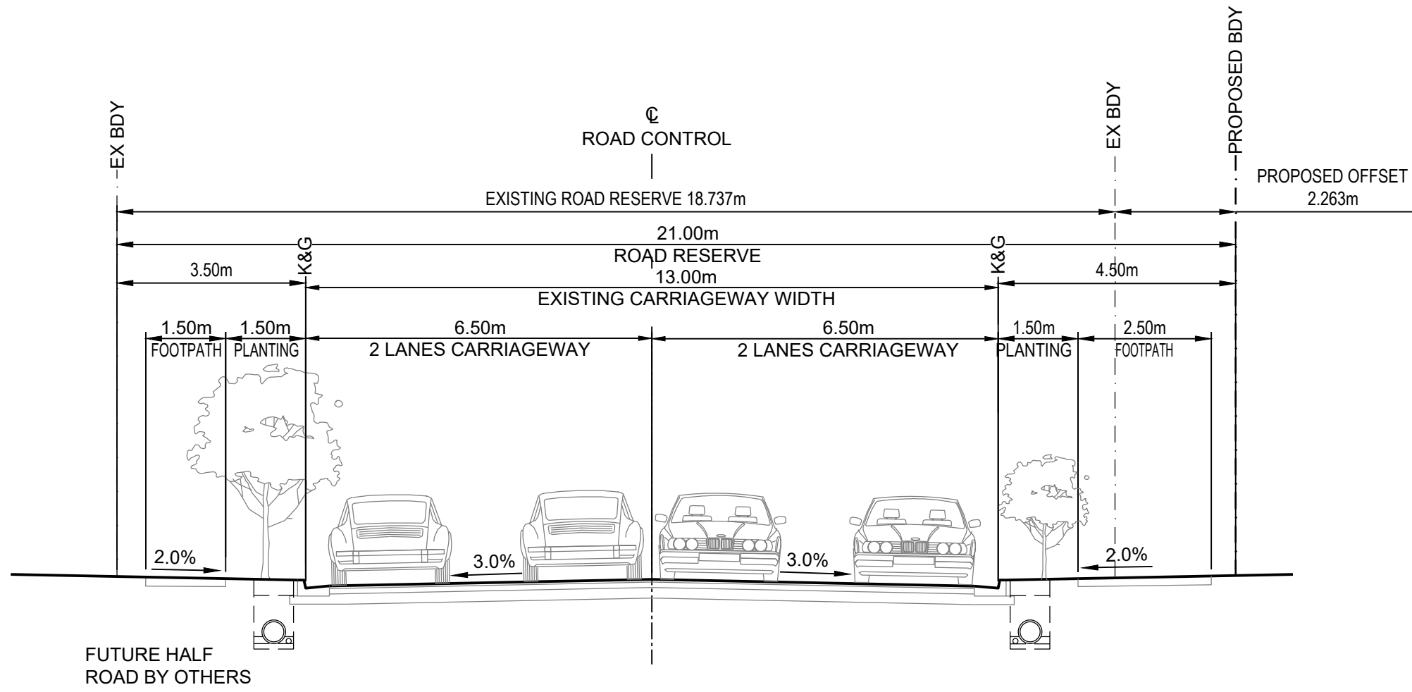
TYPICAL SECTION B - ELEVENTH AVENUE
