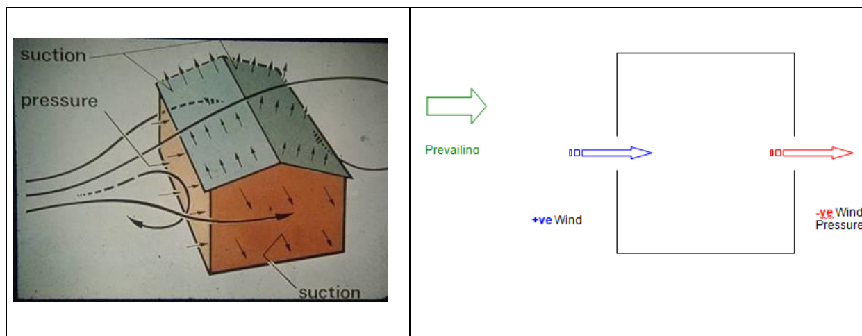
Figure 6 Wind-Induced Natural Ventilation via Differential Pressure
