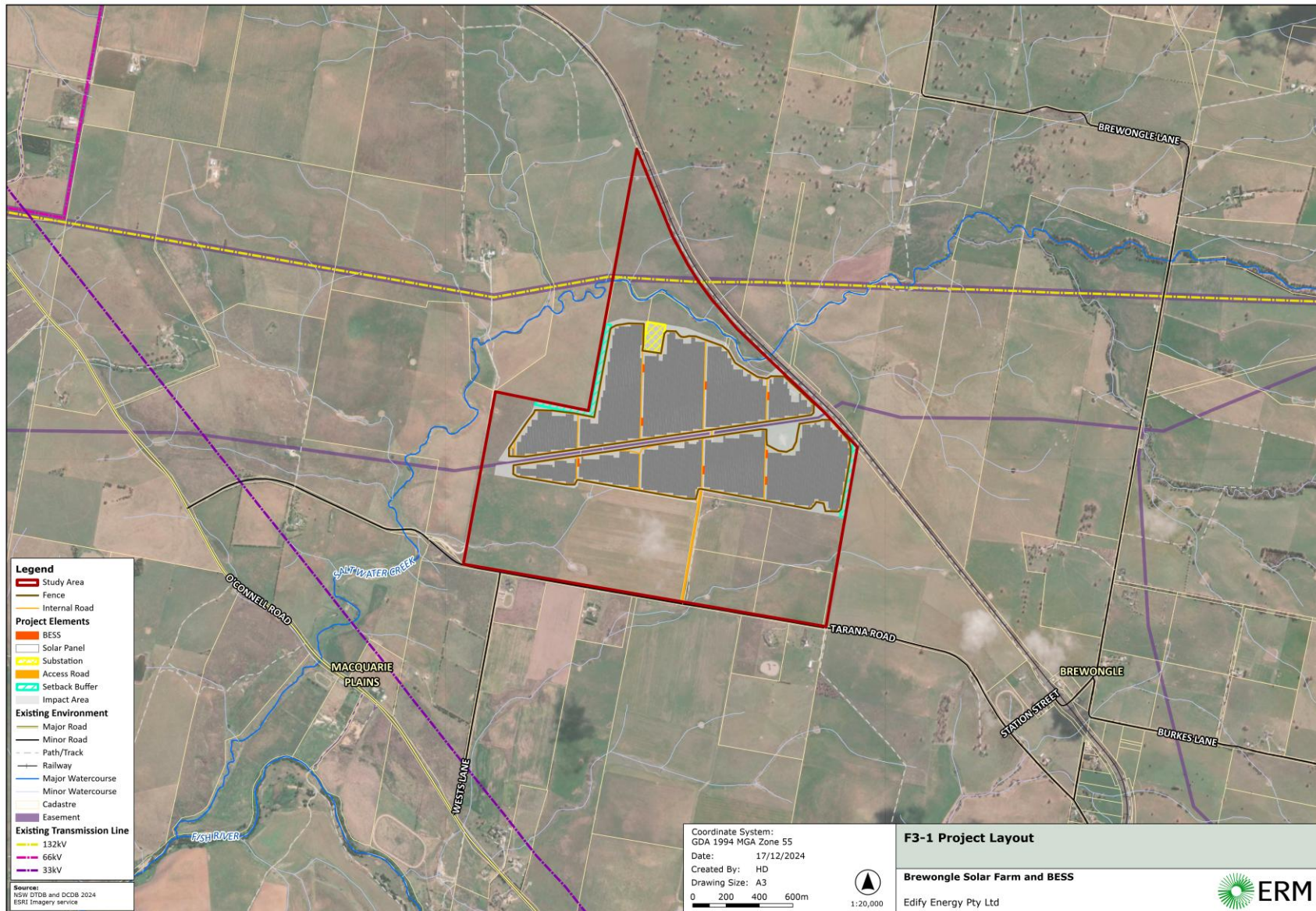
Figure 3-5: Layout
