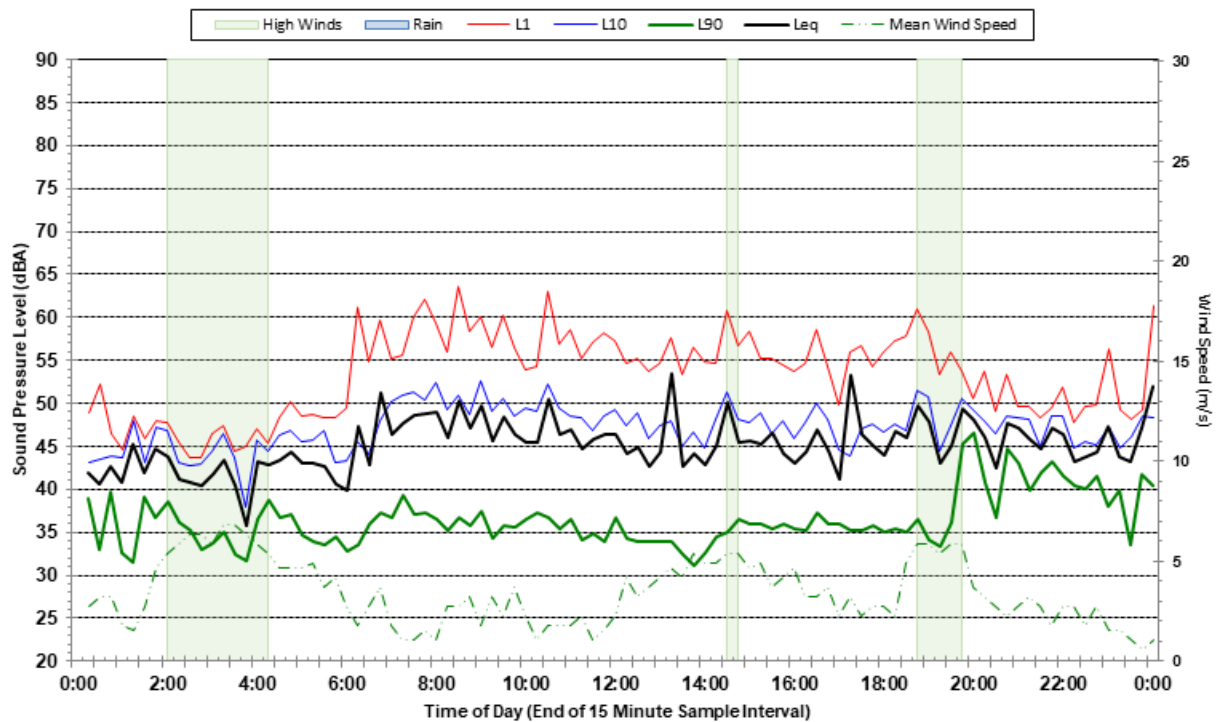
Statistical Ambient Noise Levels Western Boundary, 61 Trafalgar Avenue, Lindfield, NSW - Saturday 15 March 2025
