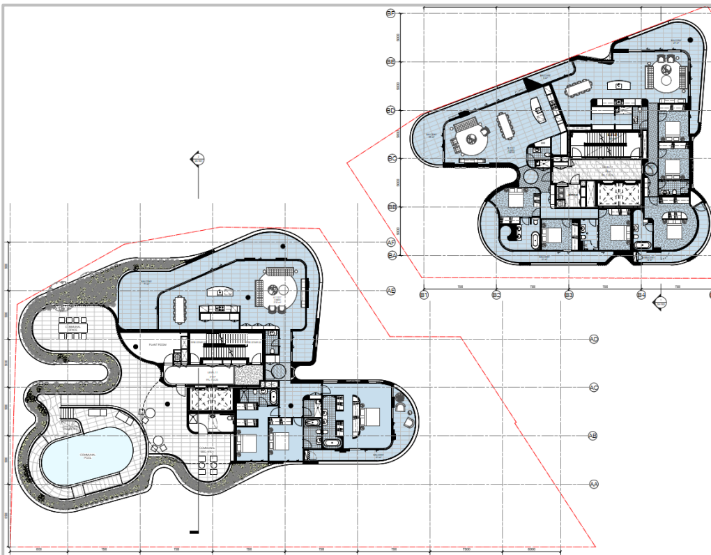
Level 11 Floor Plan
