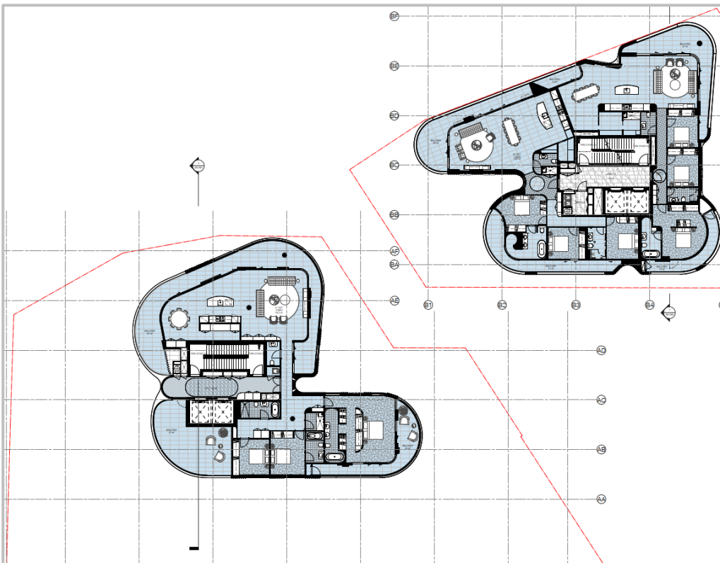
Level 13 Floor Plan
