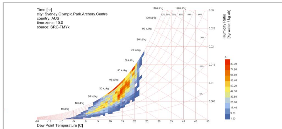
Figure 4-6 Psychrometric Chart
