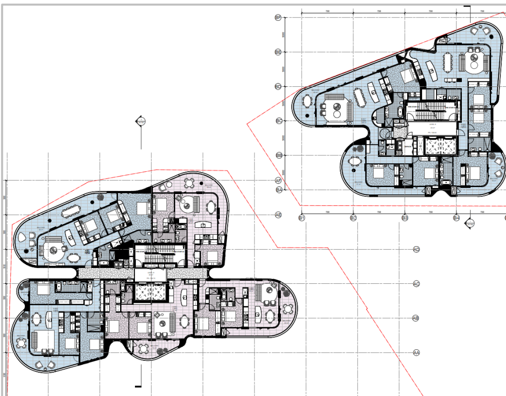
Level 9 Floor Plan
