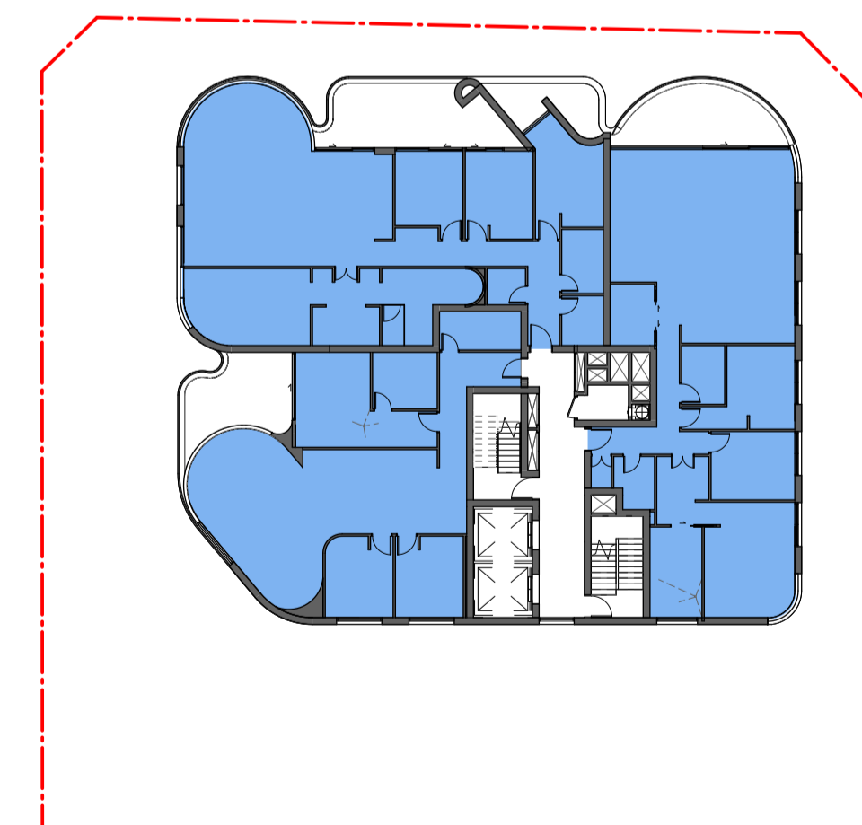
8 CROSS VENT - L4-L10 1:300
