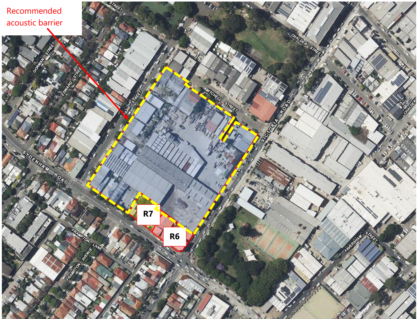
Figure 5 Recommended Acoustic Barrier
