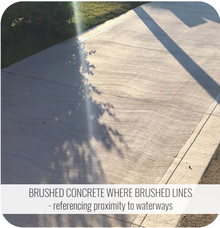
BRUSHED CONCRETE WHERE BRUSHED LINES - referencing proximity to waterways
