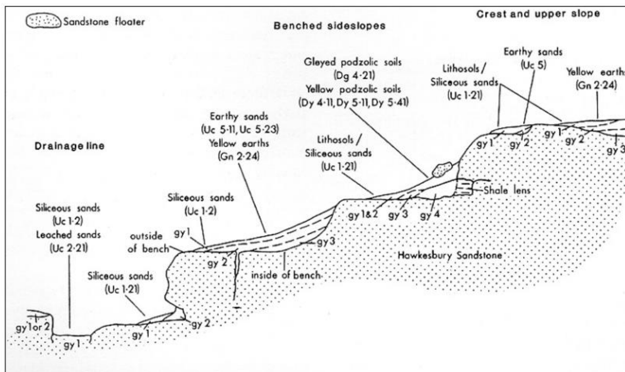
Photo 2 Schematic cross section of the Gynea soil landscape (Chapman et al. 1989, pp. 66)
