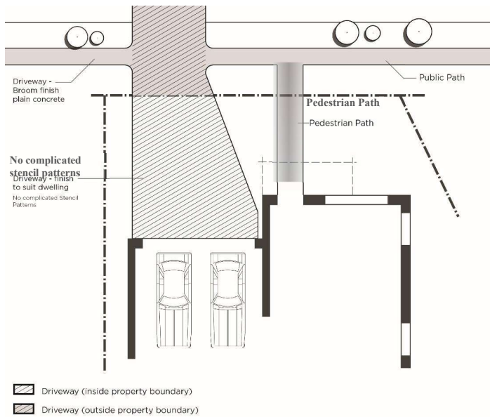
Figure 334: Driveway crossing requirements
