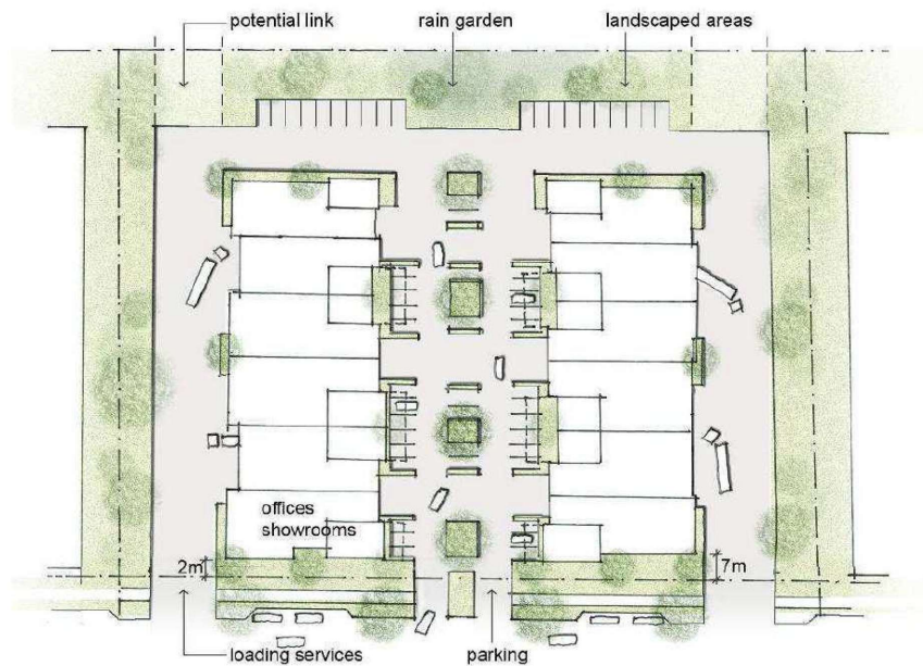
Figure 4345: Typical building layout for light industrial area
