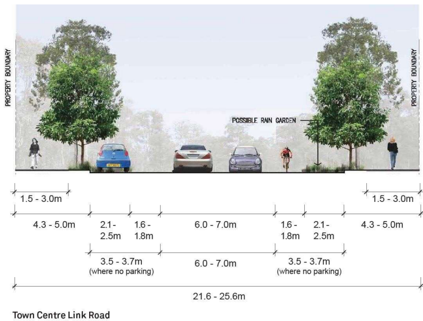
Figure 11: Town Centre Link Road
