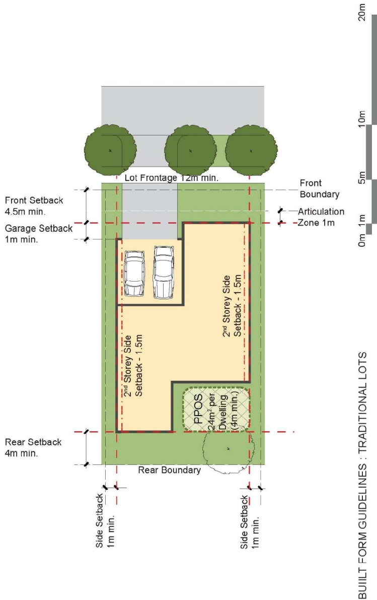
Figure 301: Indicative layout for traditional lot (detached dwelling)
