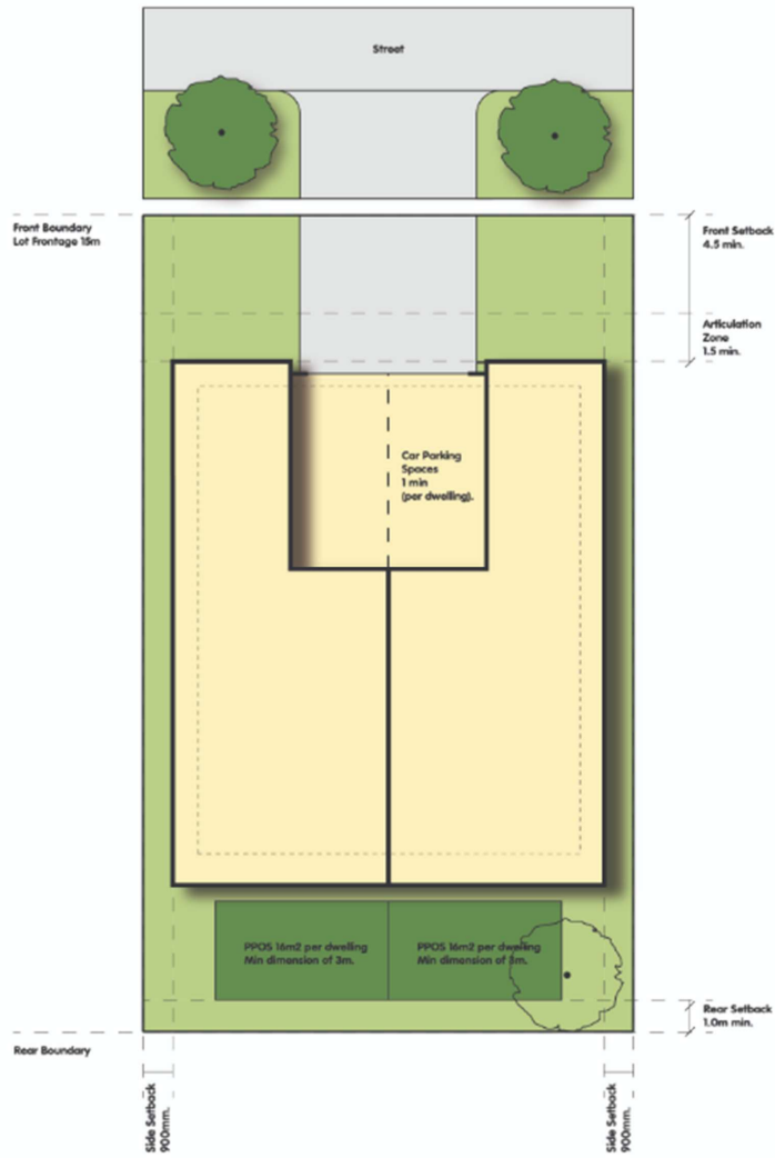
Figure #35: Indicative layout for Dual Occupancy Lots – single frontage
