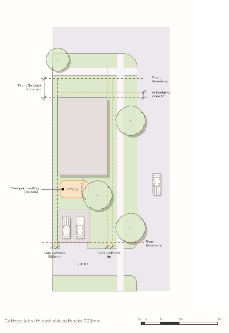
Figure 3029: Indicative layout for a cottage lot dwelling (rear loaded)
