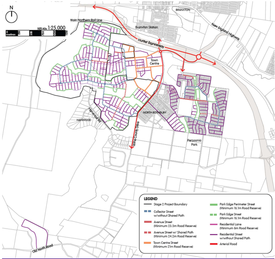
Figure 5: Overall road network and hierarchy
