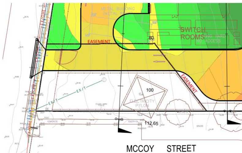
Drawing Title BULK EARTHWORKS CUT AND FILL PLAN
