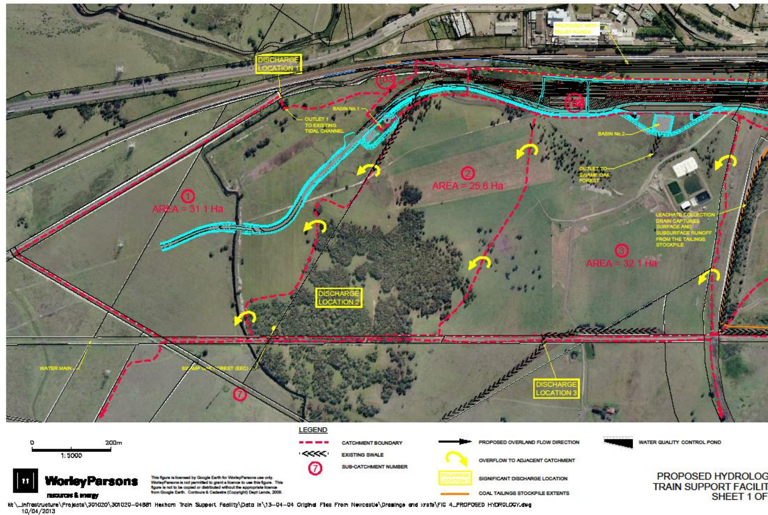
Figure 1 - Site Hydrology (a)
