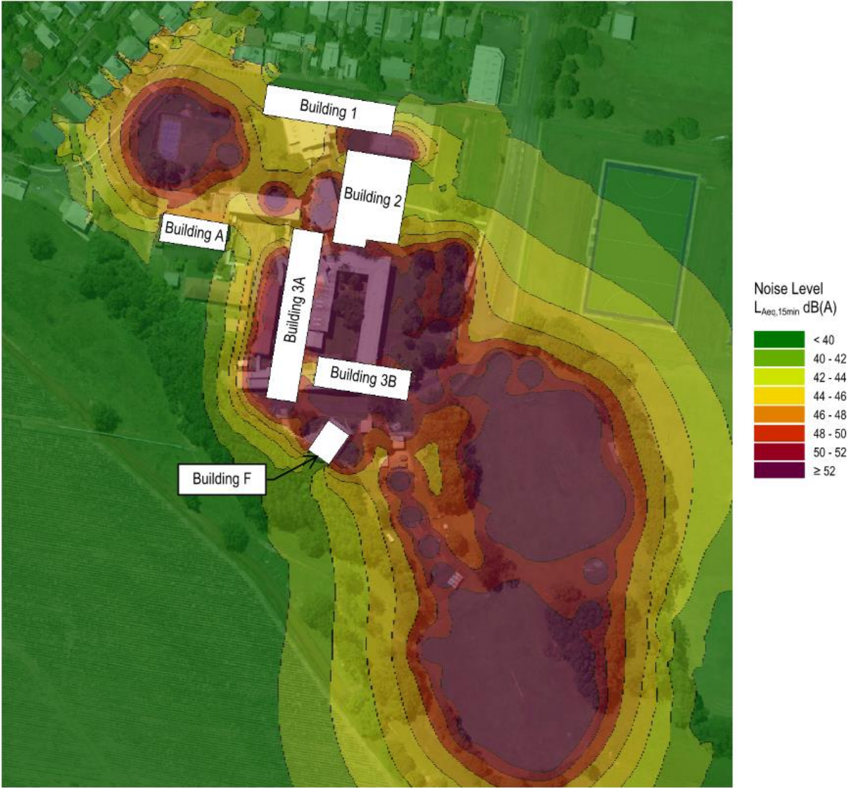
Figure 5: Noise emission map of students playing during recess and lunch
