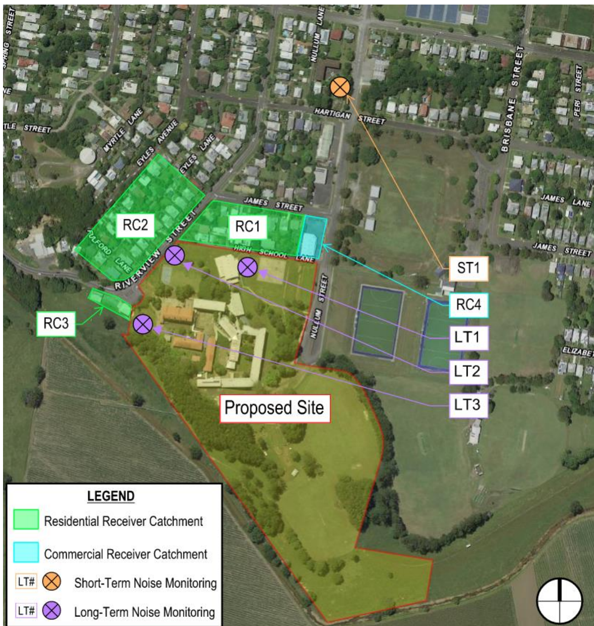
Figure 2: Overview of the site, surrounding noise-sensitive receivers and measurement locations conducted by Acoustiworks
