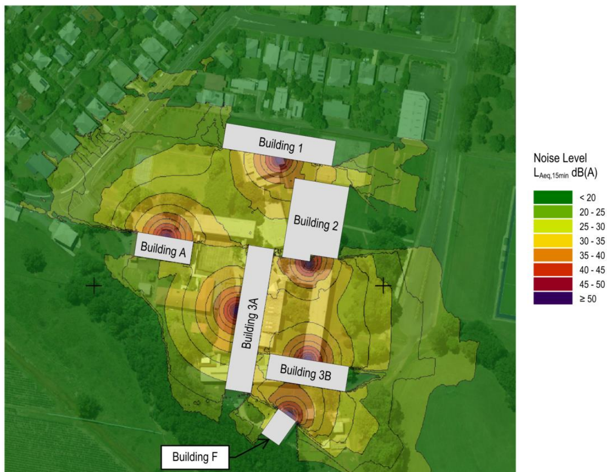
Figure 4: Noise emission map of Bells and PA systems
