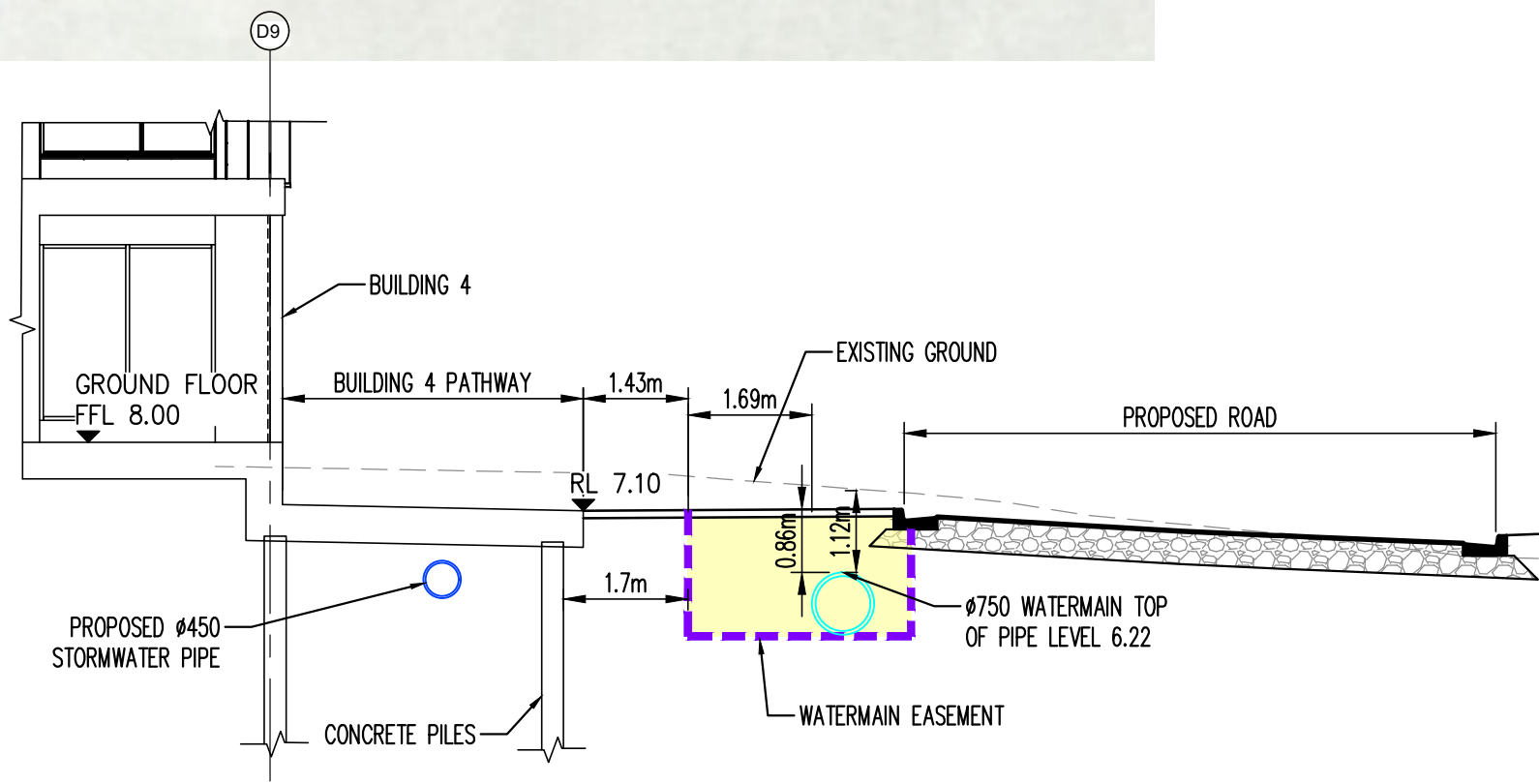
SECTION A SCALE 1:100
