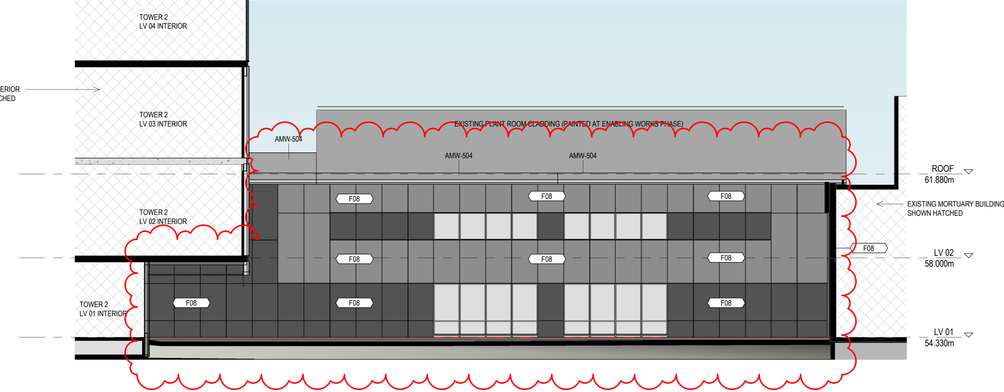
2 NORTH BLOCK - NORTH ELEVATION 1
