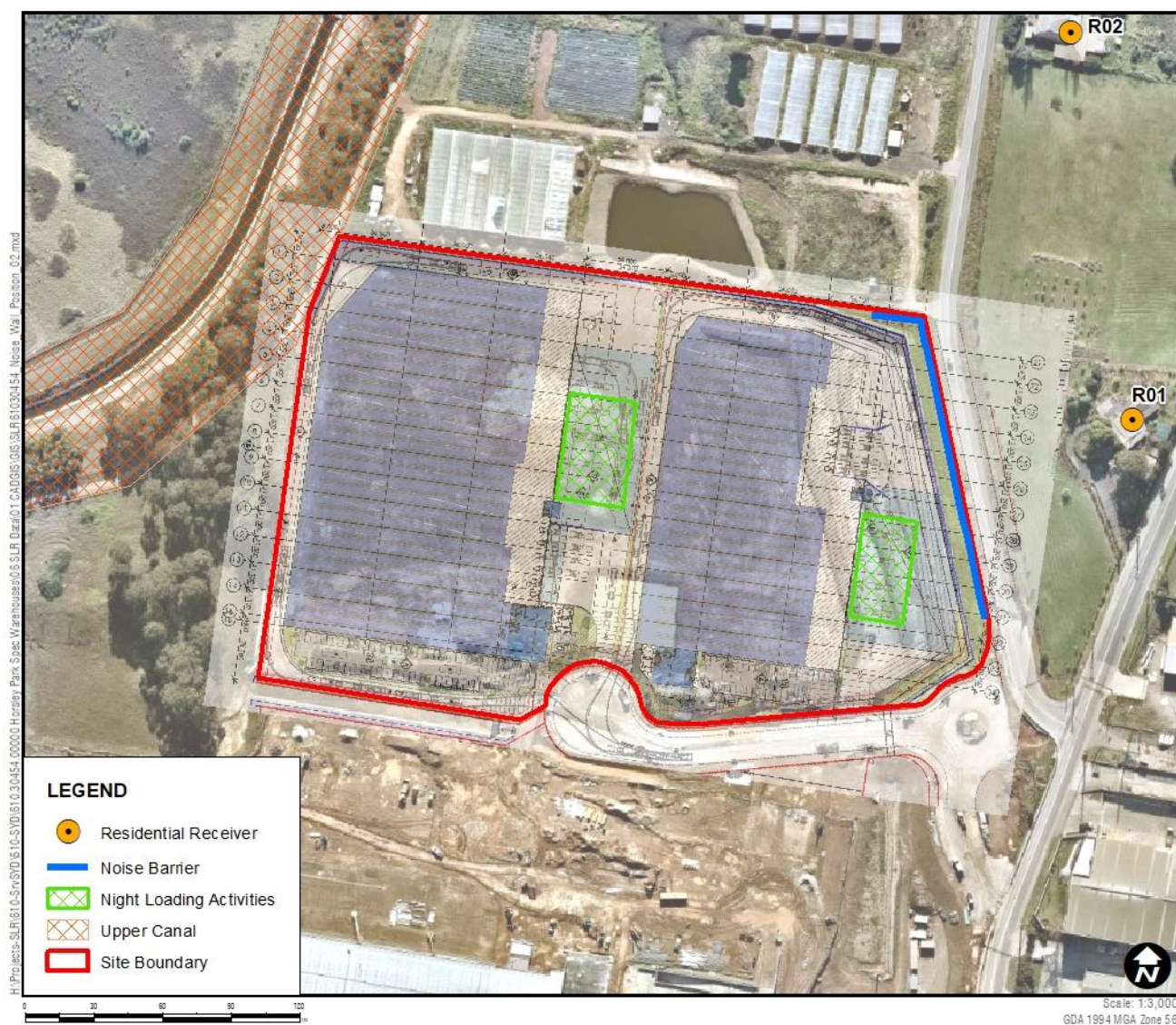
Figure 7 Recommended Noise Mitigation
