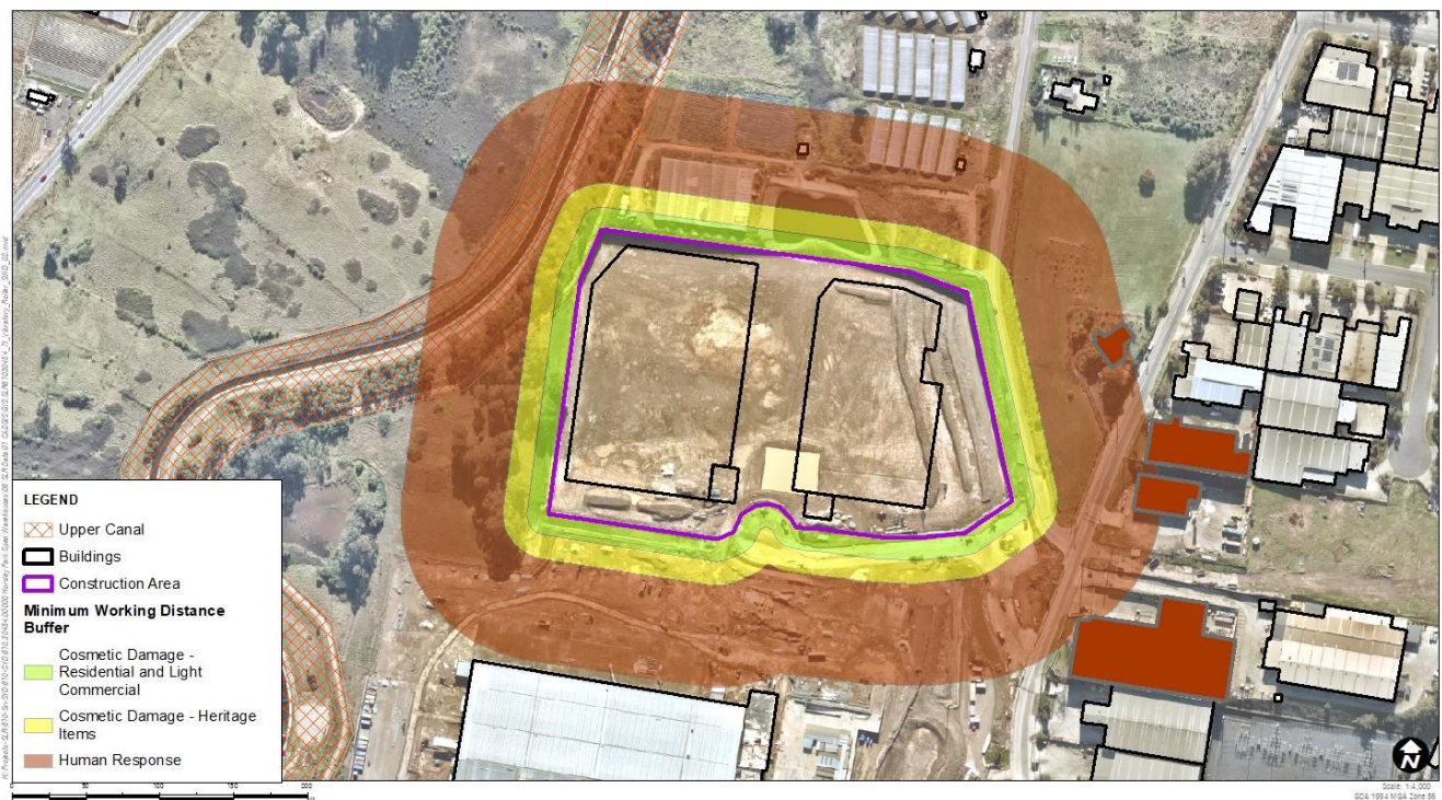
Figure 5 Construction Vibration – 7 t Vibratory Roller
