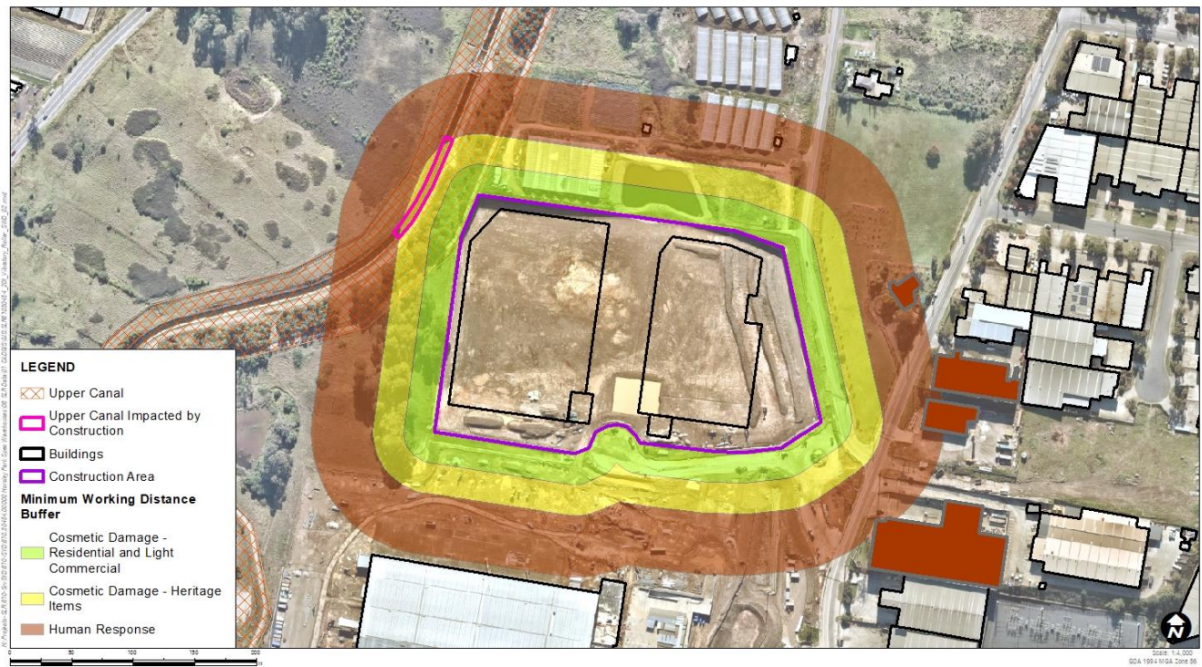
Figure 4 Construction Vibration – 20 t Vibratory Roller
