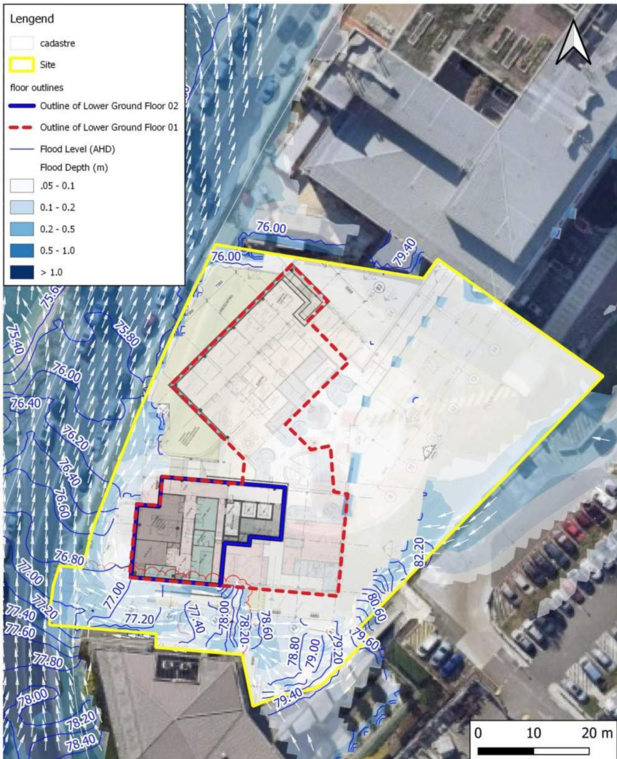
Figure 19- Flood Levels & Depths (PMF) – Proposed Conditions (Ground Floor)
