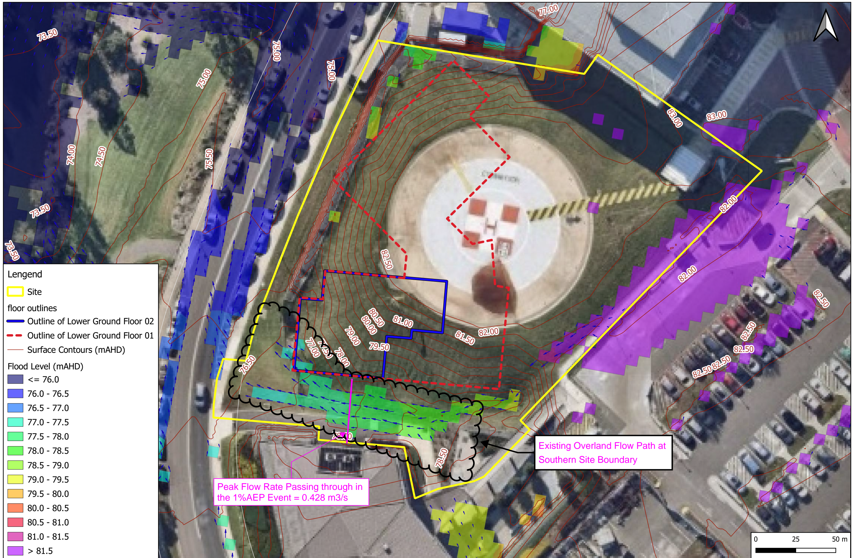
Figure A1 - Existing Overland Flow Path at Southern Site Boundary
