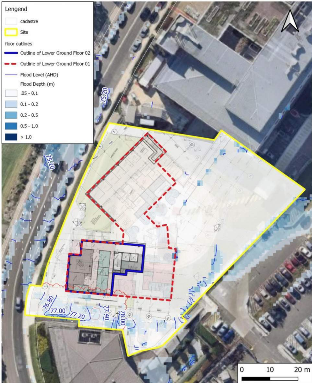
Figure 16 - Flood Levels & Depths (1% AEP) – Proposed Conditions (Ground Floor)
