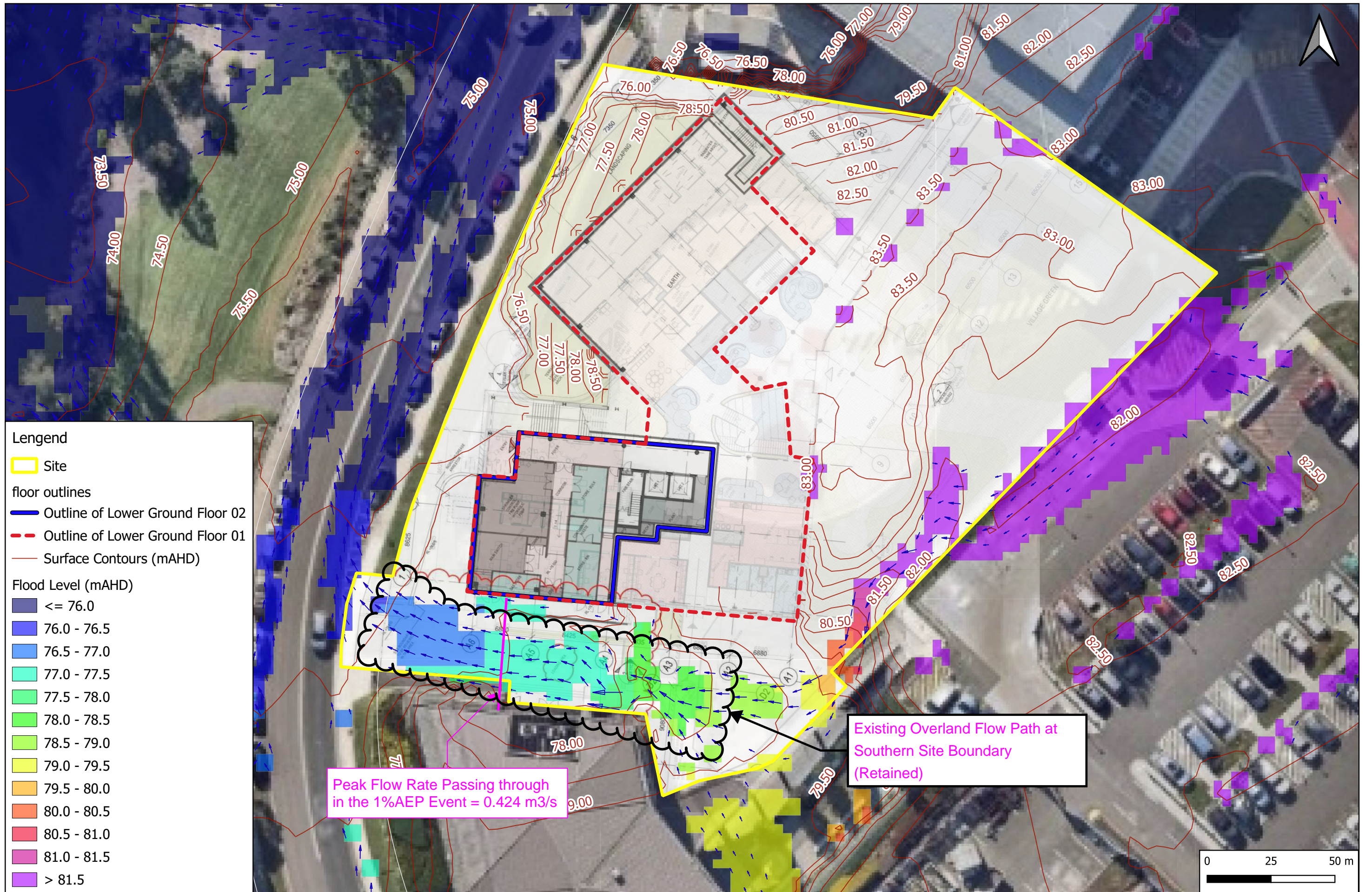
Figure A2 - Existing Overland Flow Path Retained in Post Development Conditions
