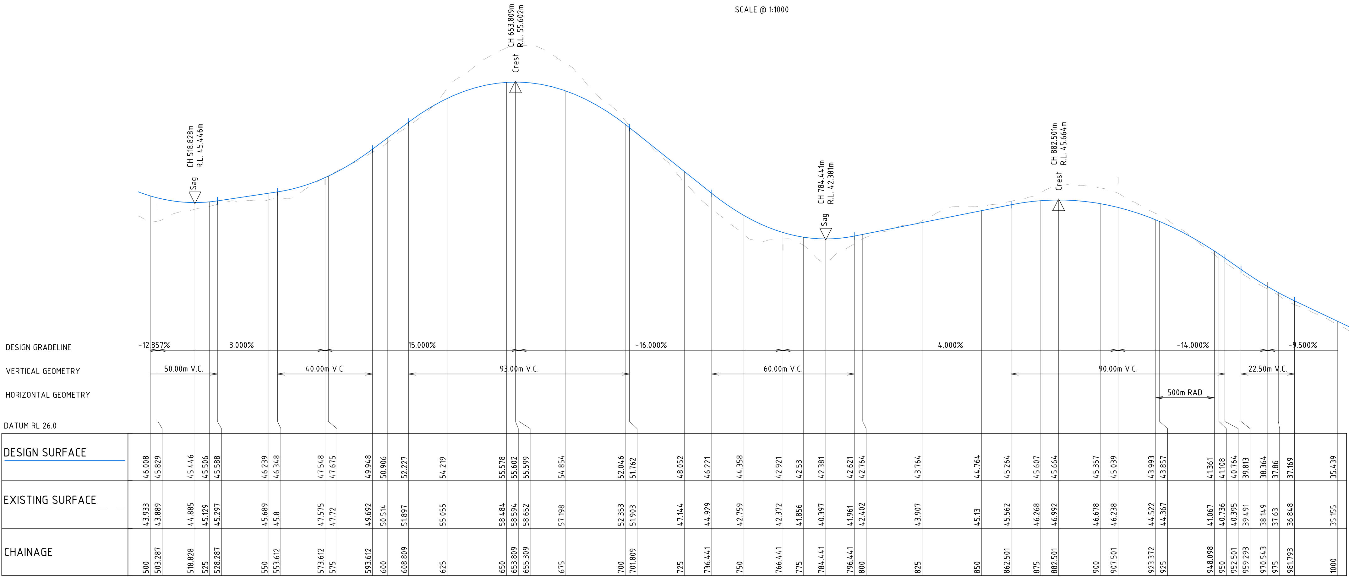
LONGITUDINAL SECTION ALONG MC11 HORIZONTAL SCALE 1:1000@A1 VERTICAL SCALE 1200@A1
