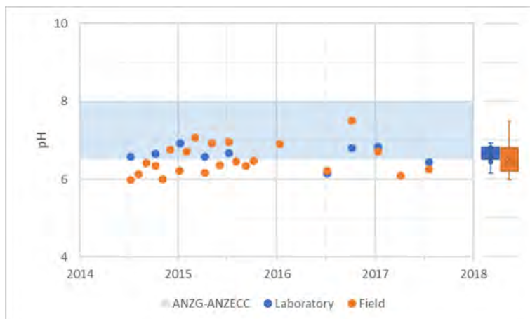
Figure 2-5: Observed pH – SOUTH
