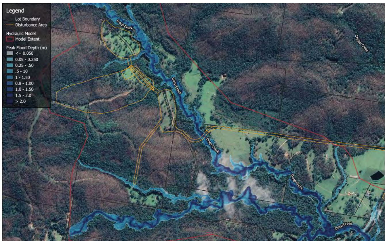
Figure 2-2: Maximum Modelling Flood Depths (1% AEP) – Existing Conditions
