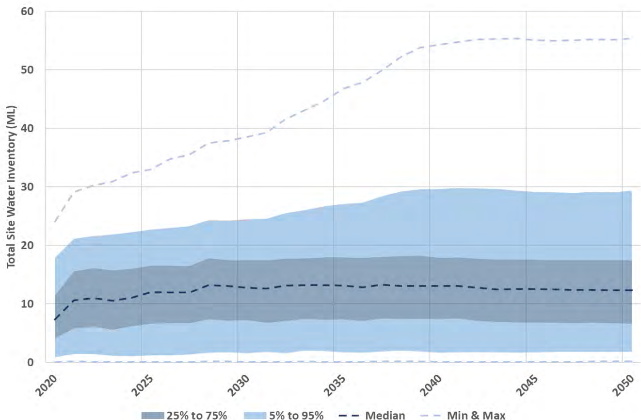
Figure 4-7: Predicted Site Water Inventory
