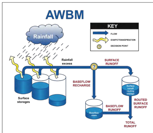
Figure 4-6: AWBM Schematic (adapted from Boughton 2004)
