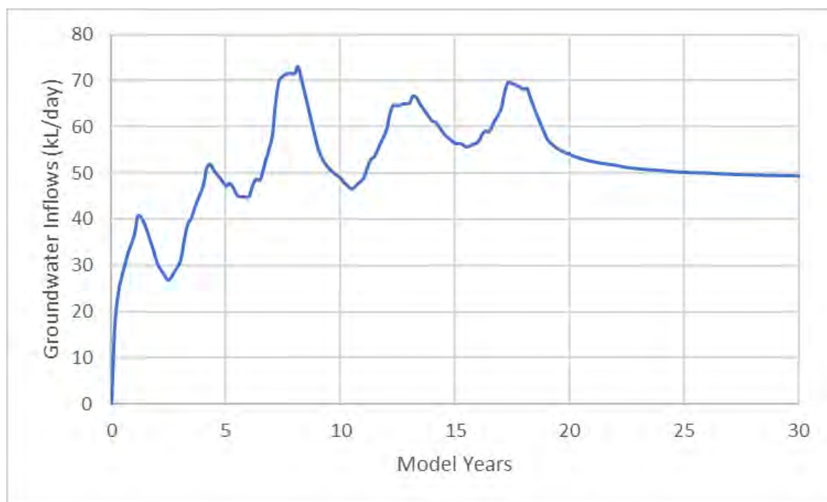
Figure 4-4: Forecast Groundwater Inflow
