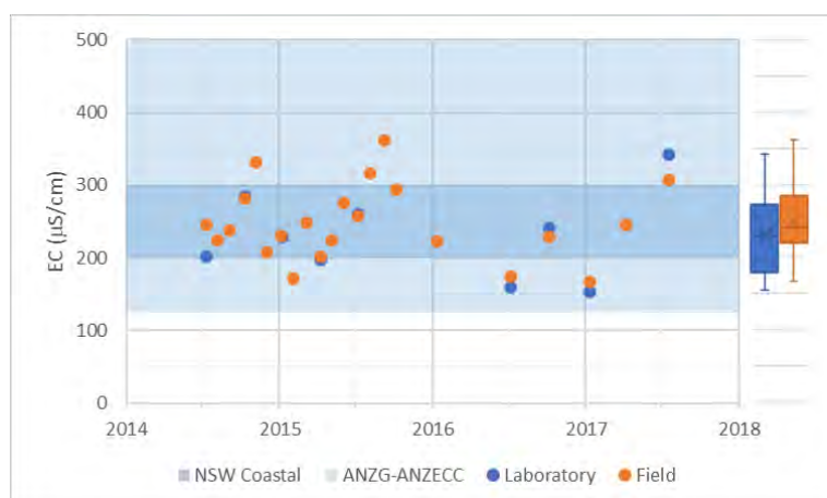
Figure 2-9: Observed EC – SOUTH
