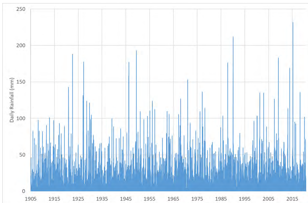
Figure 4-2: Historical SILO Rainfall Data
