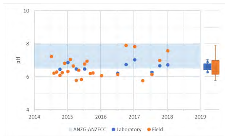
Figure 2-6: Observed pH – DAM
