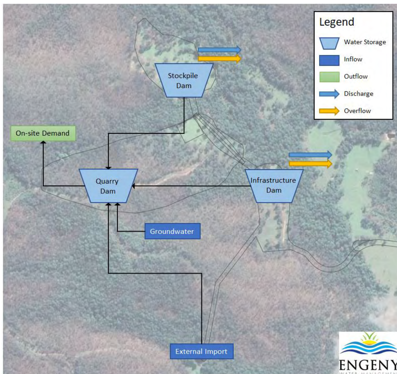
Figure 4-1: Water Balance Model Schematic
