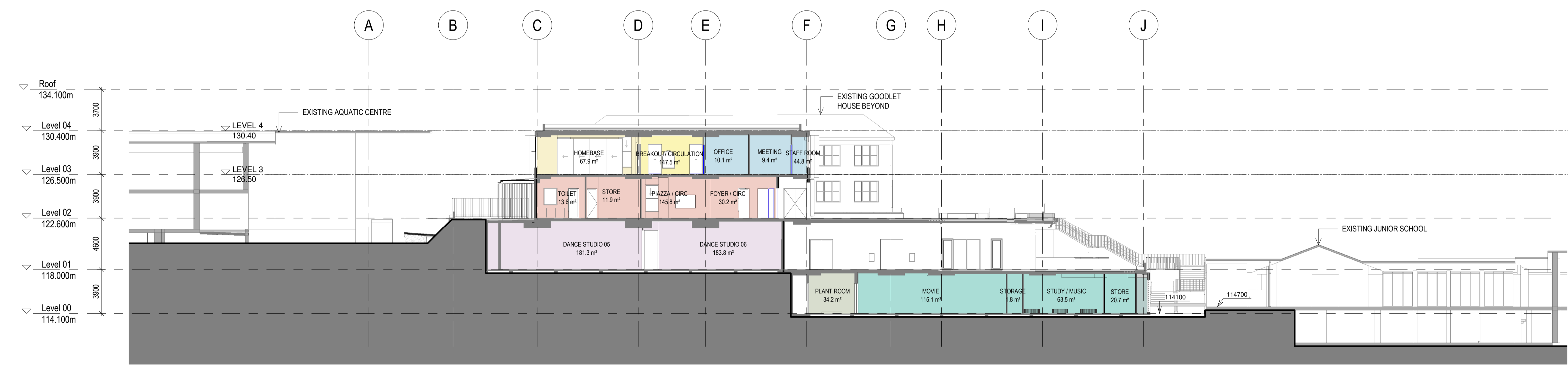
2 EAST / WEST SECTION 2 1 : 200
