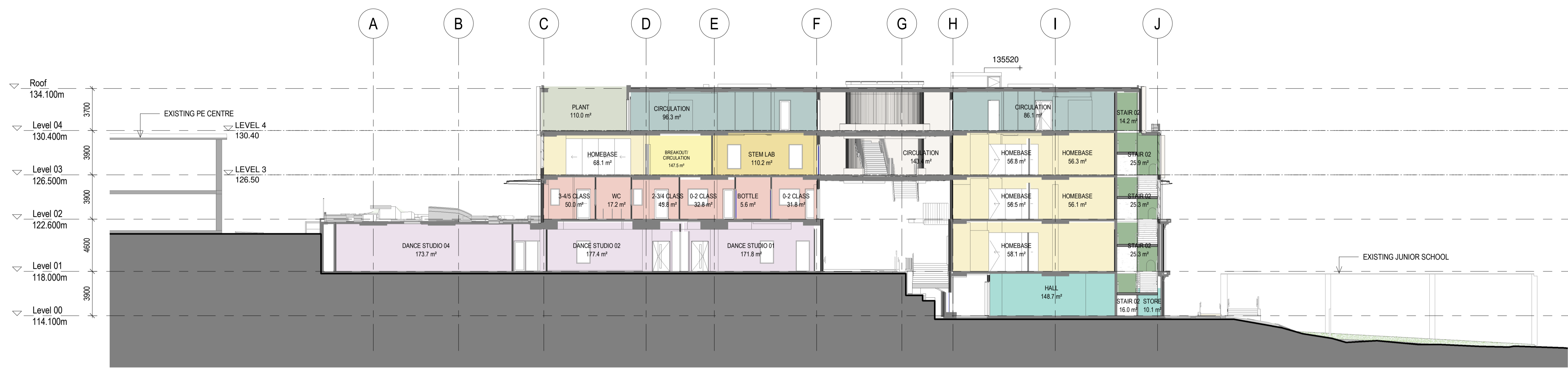
1 EAST / WEST SECTION 1 1 : 200
