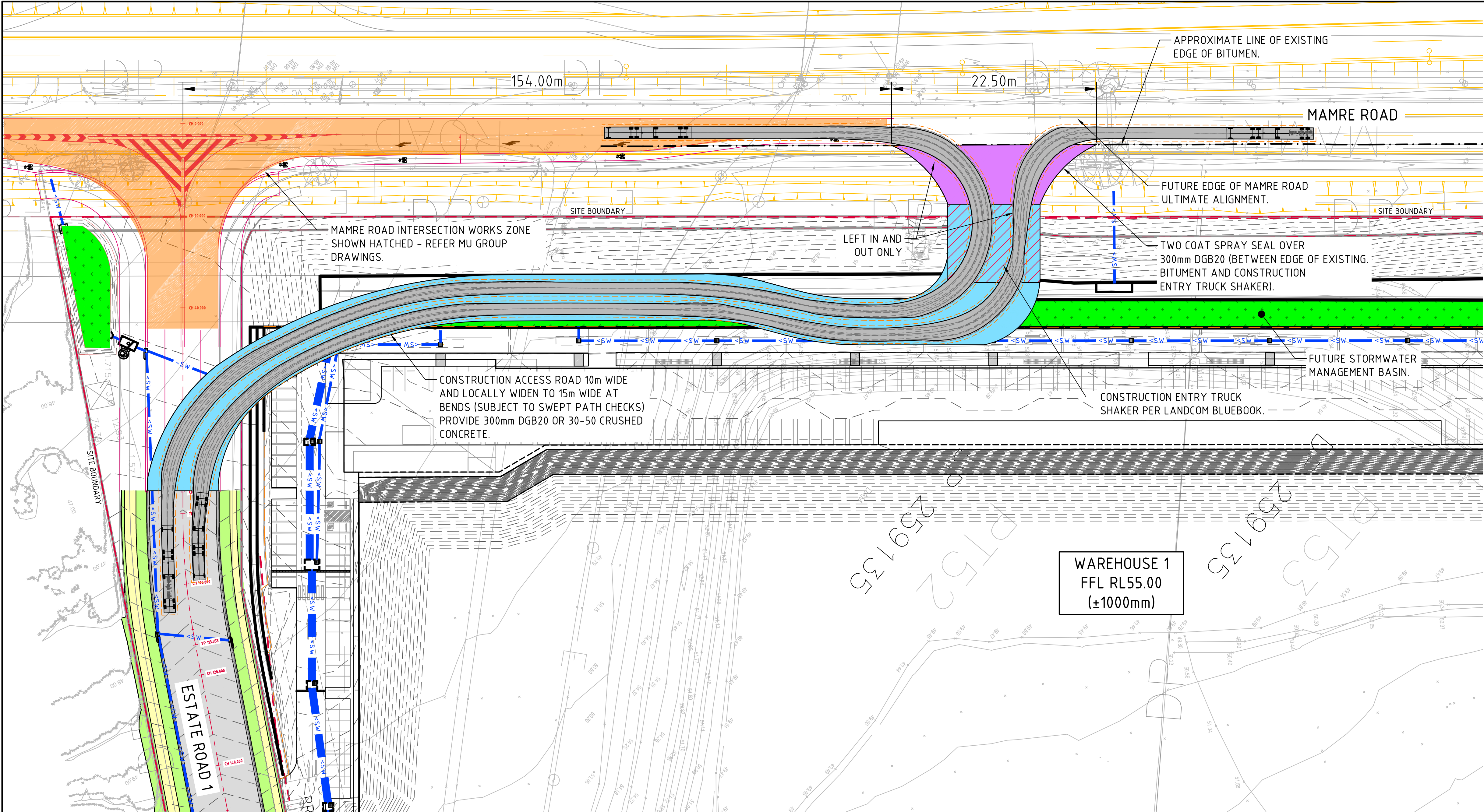
TEMPORARY ENTRY PLAN - SHEET 2 SCALE 1:500
