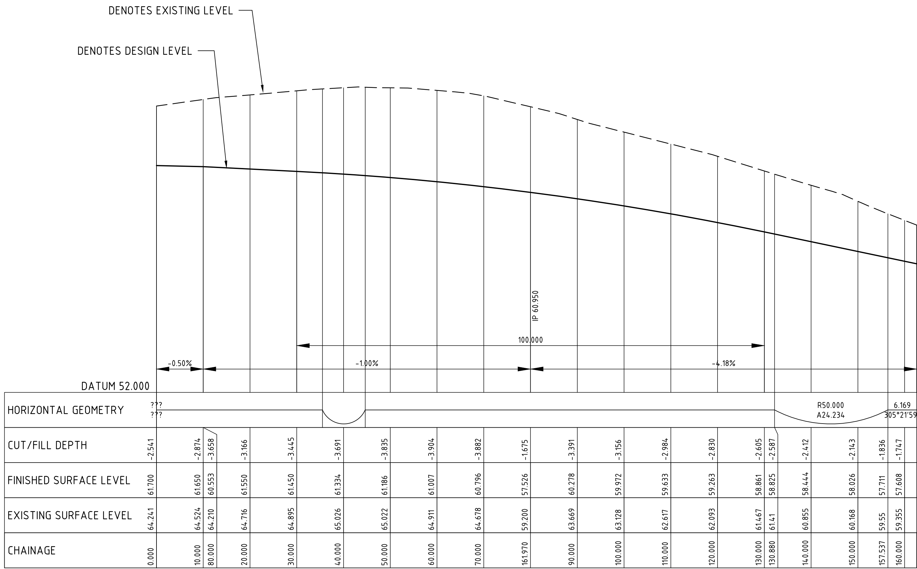
LONGITUDINAL SECTION - CL DIST RD 2 HORIZONTAL SCALE 1:500 VERTICAL SCALE 1:100
