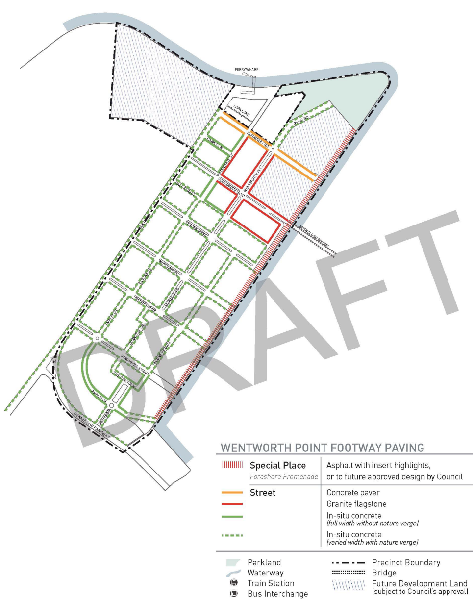
Figure 4.61 Wentworth Point Urban Village - Paving Strategy
