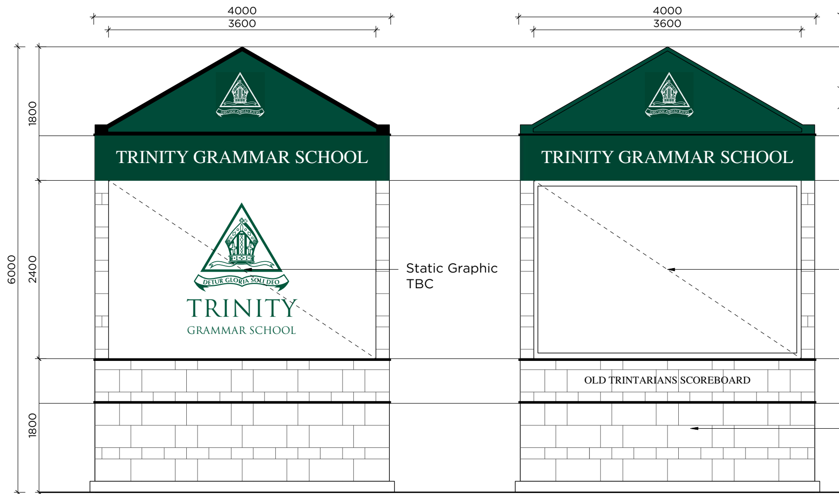
03 Oval Facing Facade Scale: 1:50
