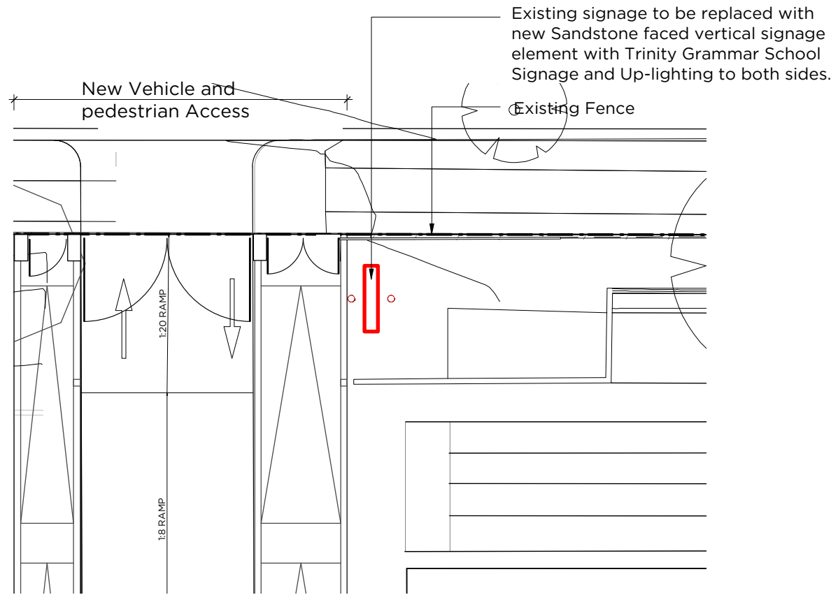
01 Victoria Street entry signage plan Scale: 1:200
