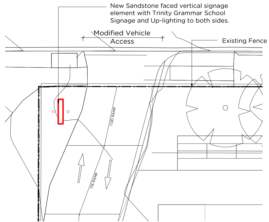
02 Victoria Street entry signage plan Scale: 1:200
