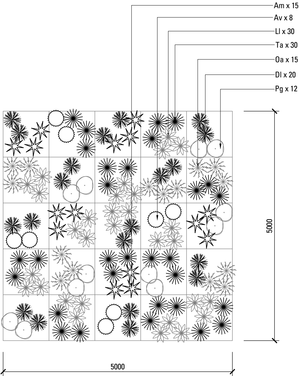
01 NATIVE GRASSES + GROUNDCOVER MATRIX - 5m x 5m SCALE 1:50 NOTE: DETAIL IS INDICATIVE ONLY, PLANT ALL SPECIES RANDOMLY AT AM OVERALL RATE OF 6/m 2
