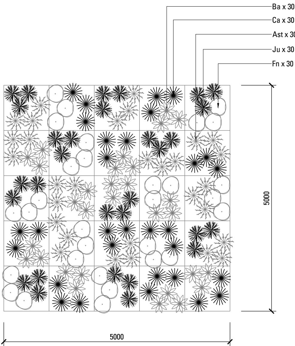
03 SWALE MATRIX - 5m x 5m SCALE 1:50 NOTE: DETAIL IS INDICATIVE ONLY, PLANT ALL SPECIES RANDOMLY AT AM OVERALL RATE OF 6/m 2
