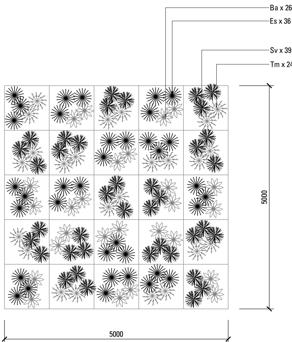
06 BIORETENTION MATRIX - 5m x 5m SCALE 1:50 NOTE: DETAIL IS INDICATIVE ONLY, PLANT ALL SPECIES RANDOMLY AT AM OVERALL RATE OF 6/m 2
