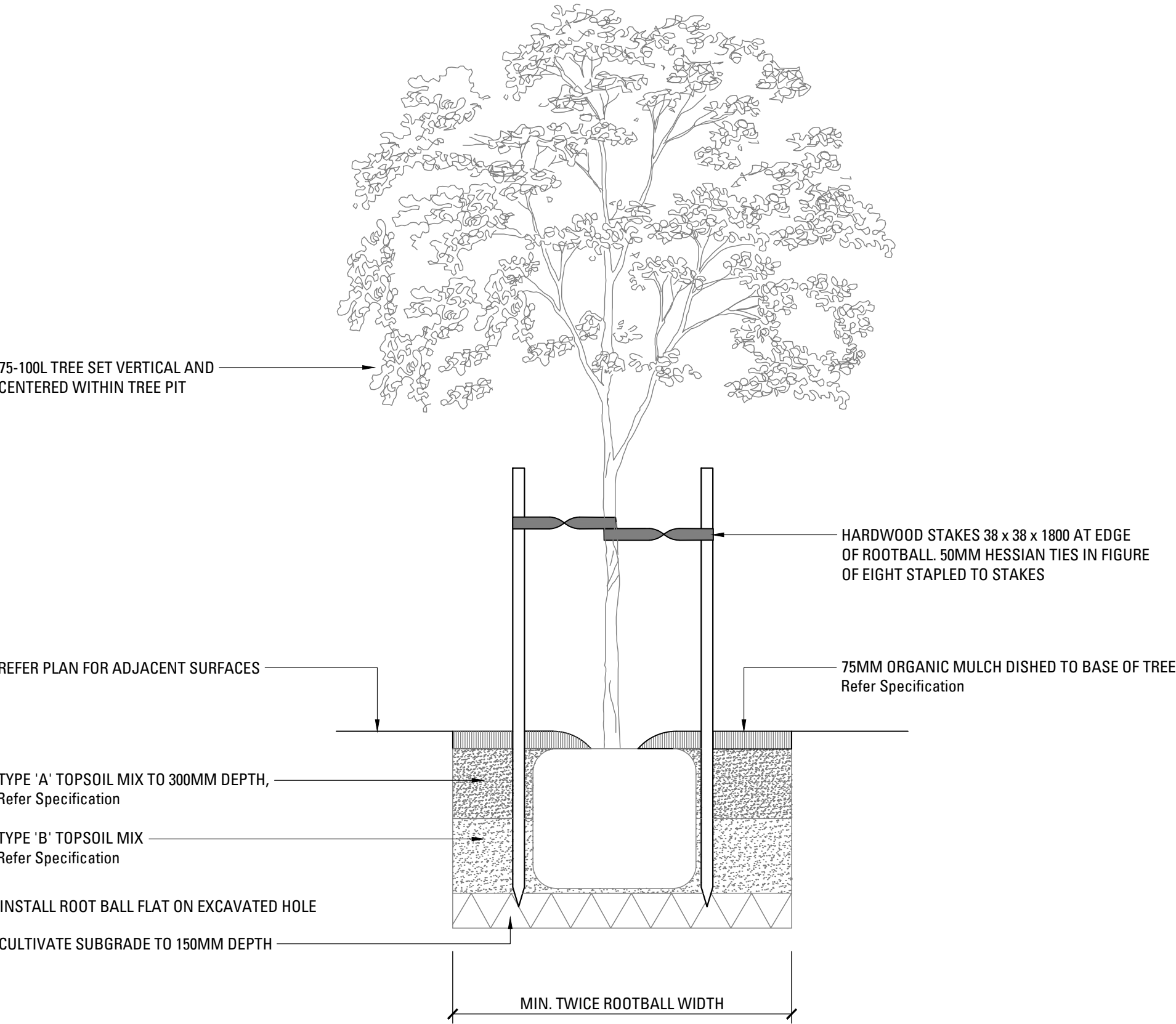
04 TREE PLANTING 75-100L SCALE 1:20
