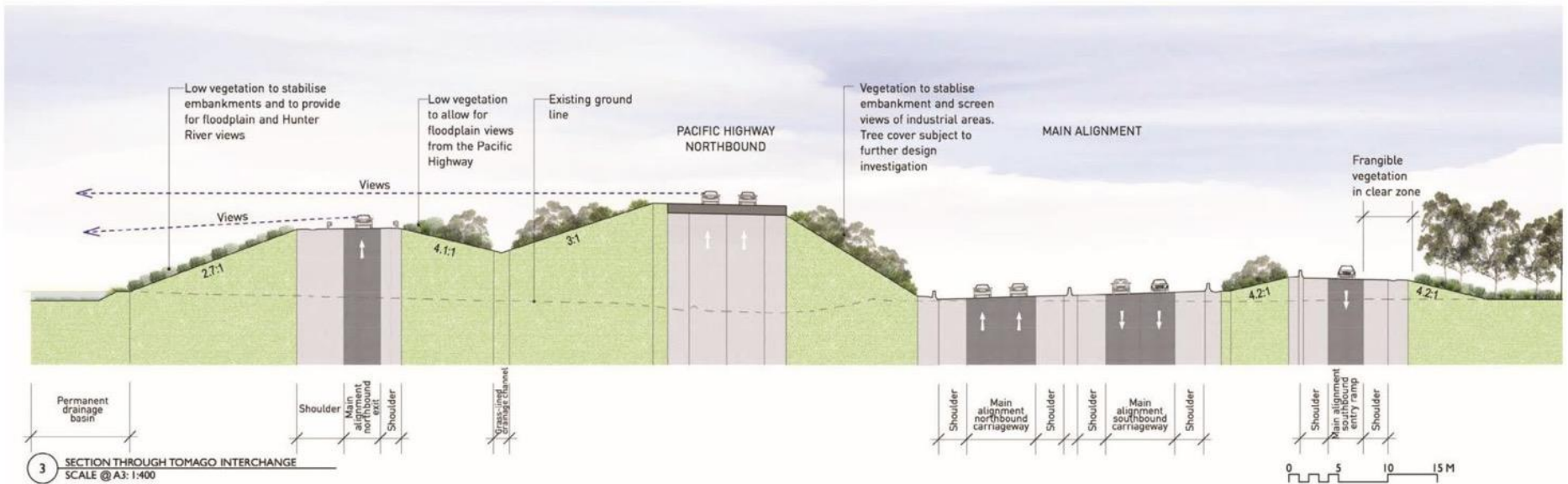
Figure 5-19 Indicative drawing of Tomago interchange section
