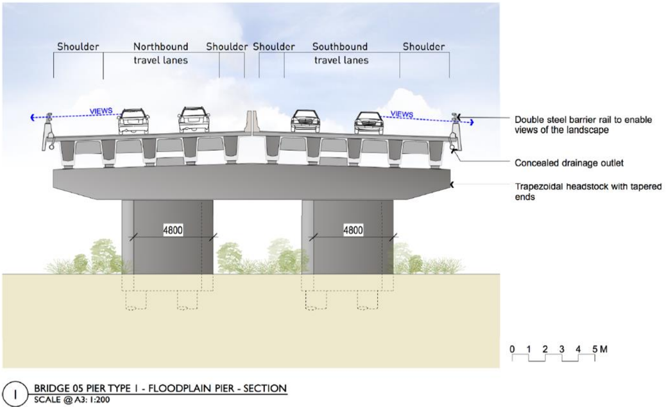
Figure 5-13 Indicative drawing of super-T girder bridge structure (B05)
