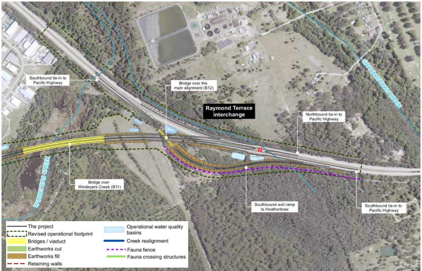
Figure 5-8 Raymond Terrace interchange configuration
