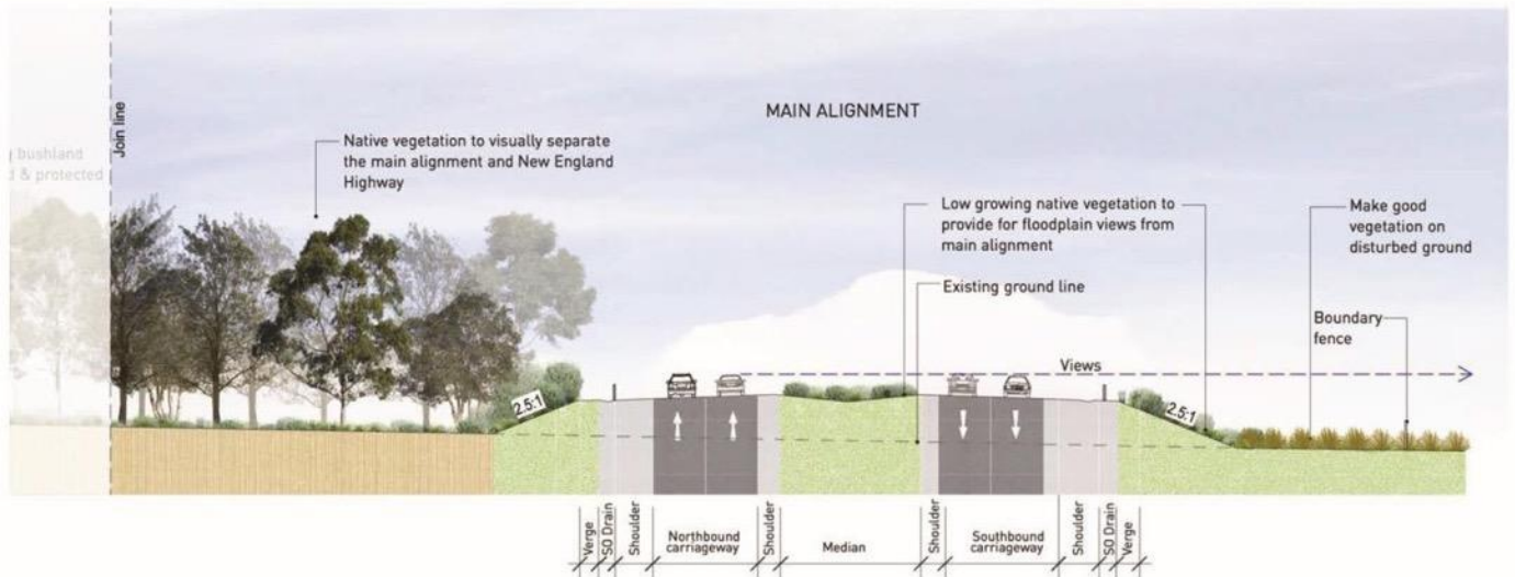
Figure 5-18 Indicative drawing of Tarro section
