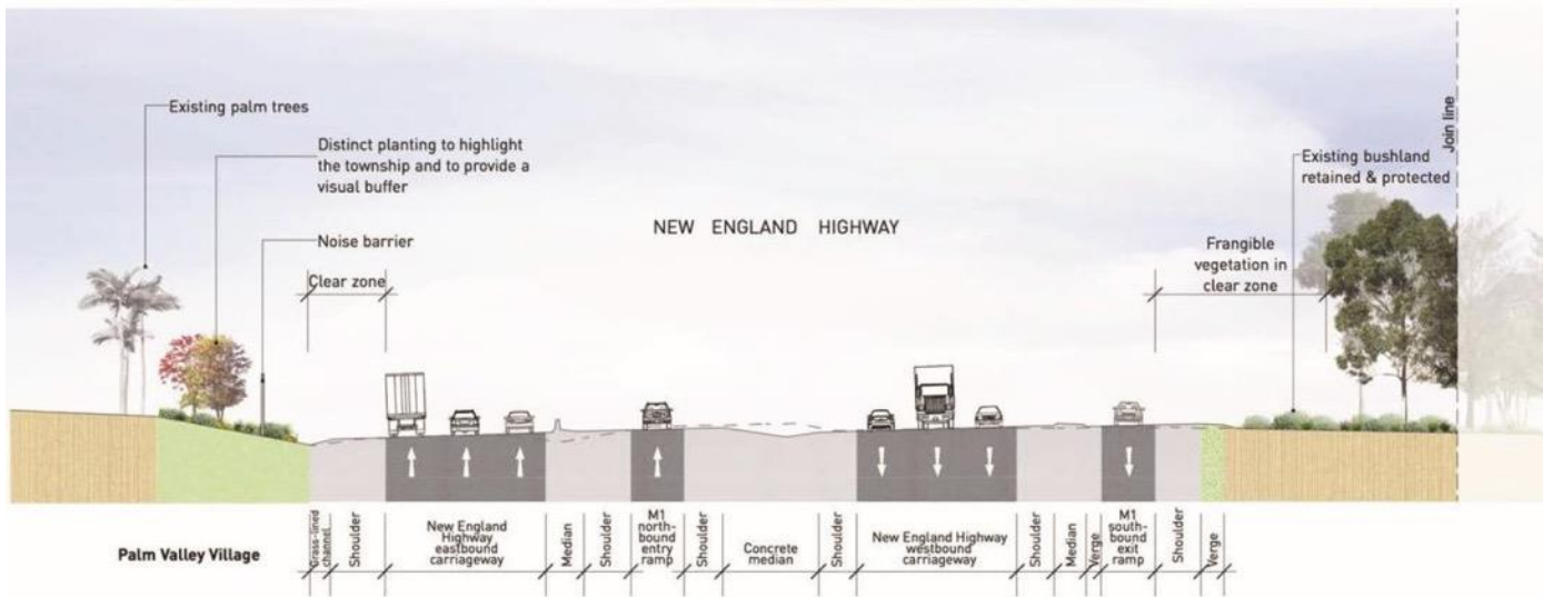
2 SECTION AT TARRO SCALE @ A3: 1:400
