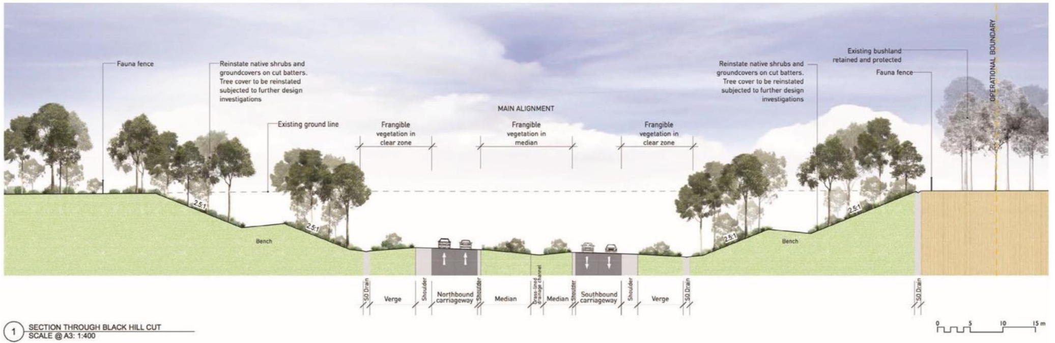
Figure 5-17 Indicative drawing of Black Hill section
