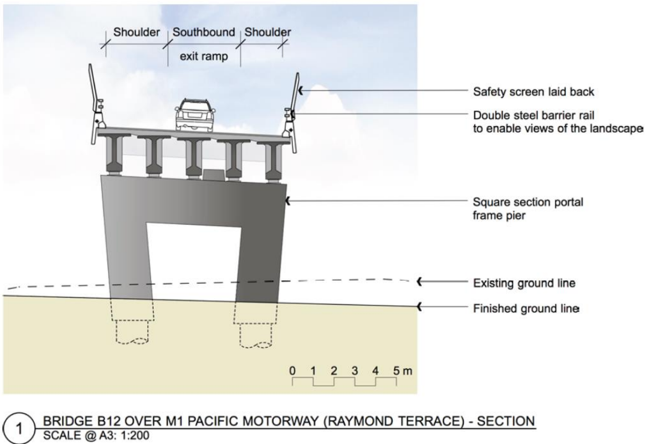
Figure 5-14 Indicative drawing of a bulb-T girder bridge structure (B12)
