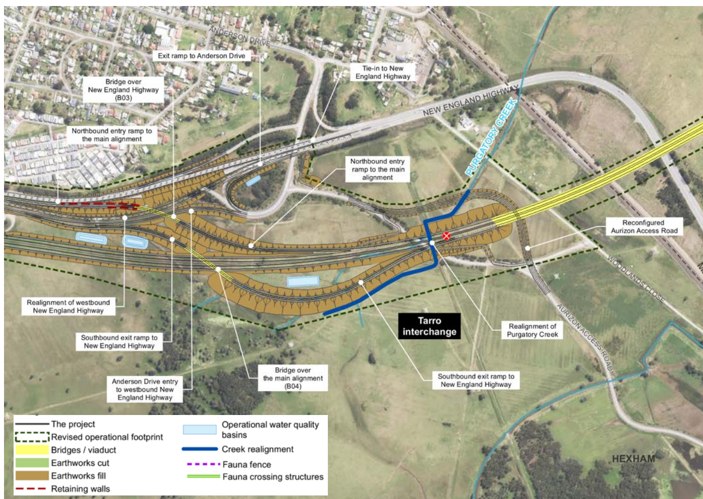
Figure 5-4 Tarro interchange configuration
