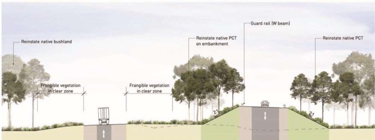
Figure 5-21 Indicative drawing of Raymond Terrace interchange section
