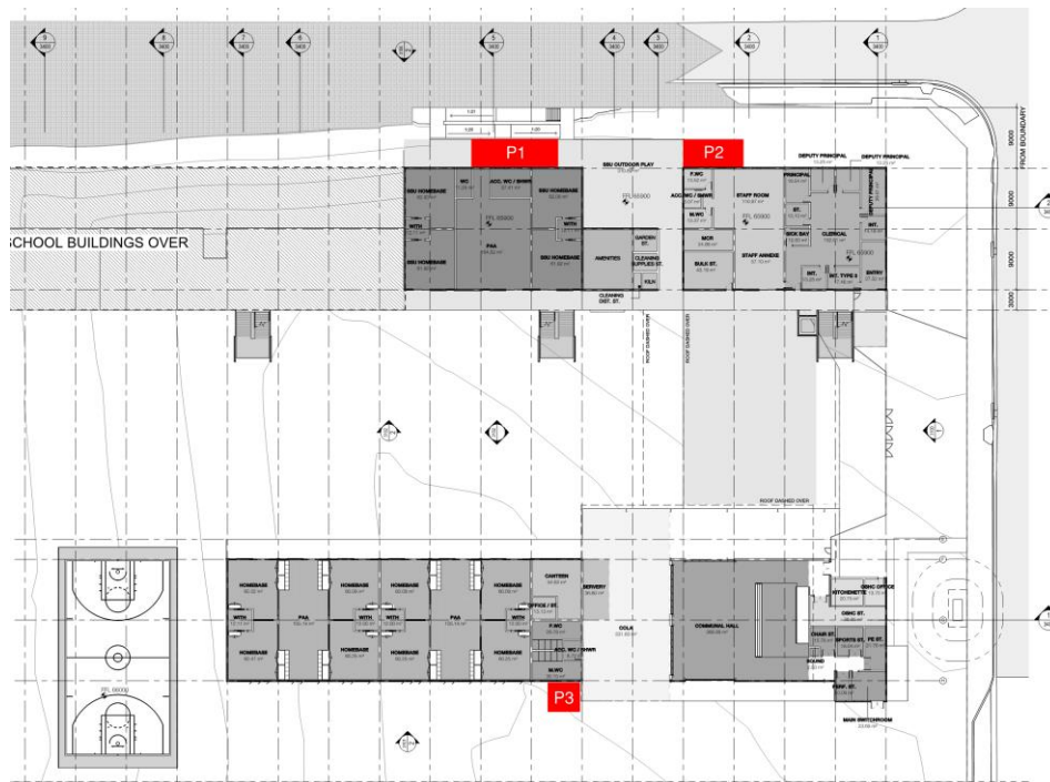
Figure 9: Proposed location of the external mechanical plants.
