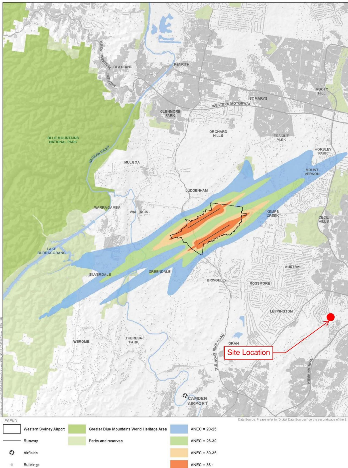
ES 19 - ANEC contours for Prefer 05 and Prefer 23 operating strategy (2063)
