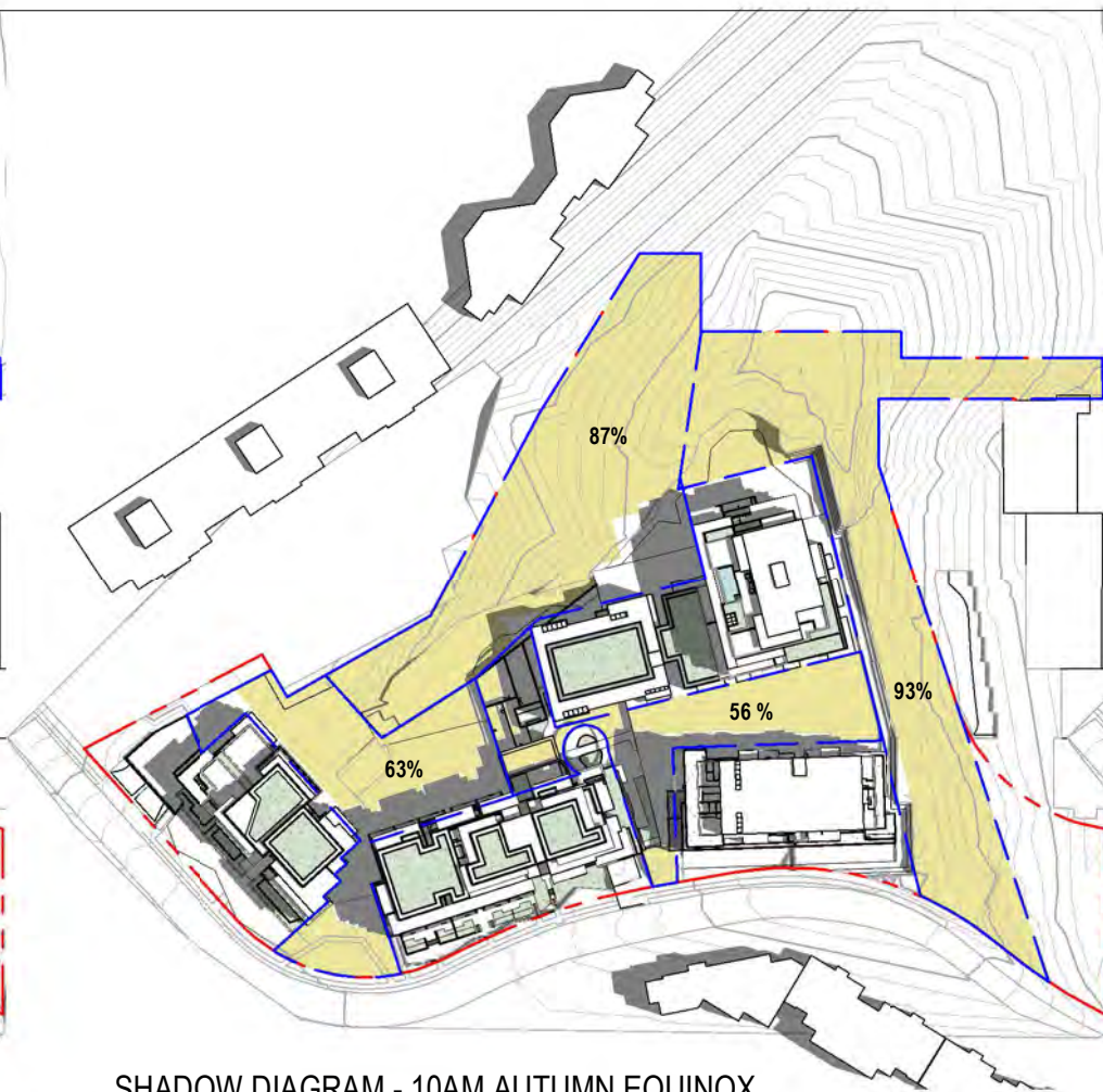
SHADOW DIAGRAM - 10AM AUTUMN EQUINOX
