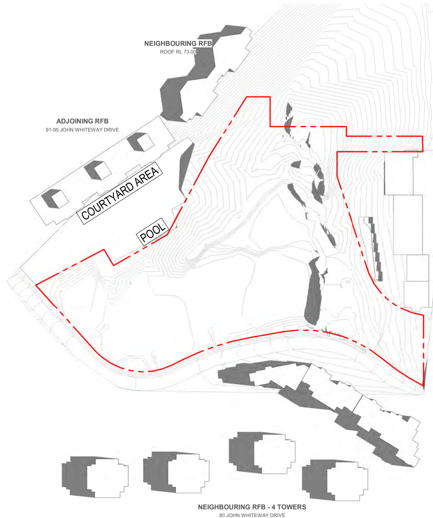
1 IMPACT ON NEIGHBOURING BUILDINGS- 11AM 21 JUNE EXISTING 1 : 1500
