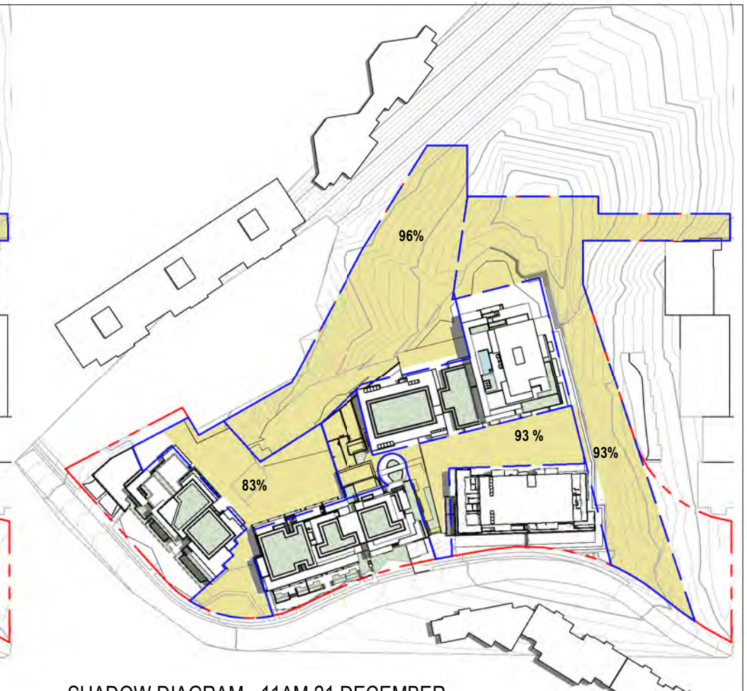
SHADOW DIAGRAM - 11AM 21 DECEMBER
