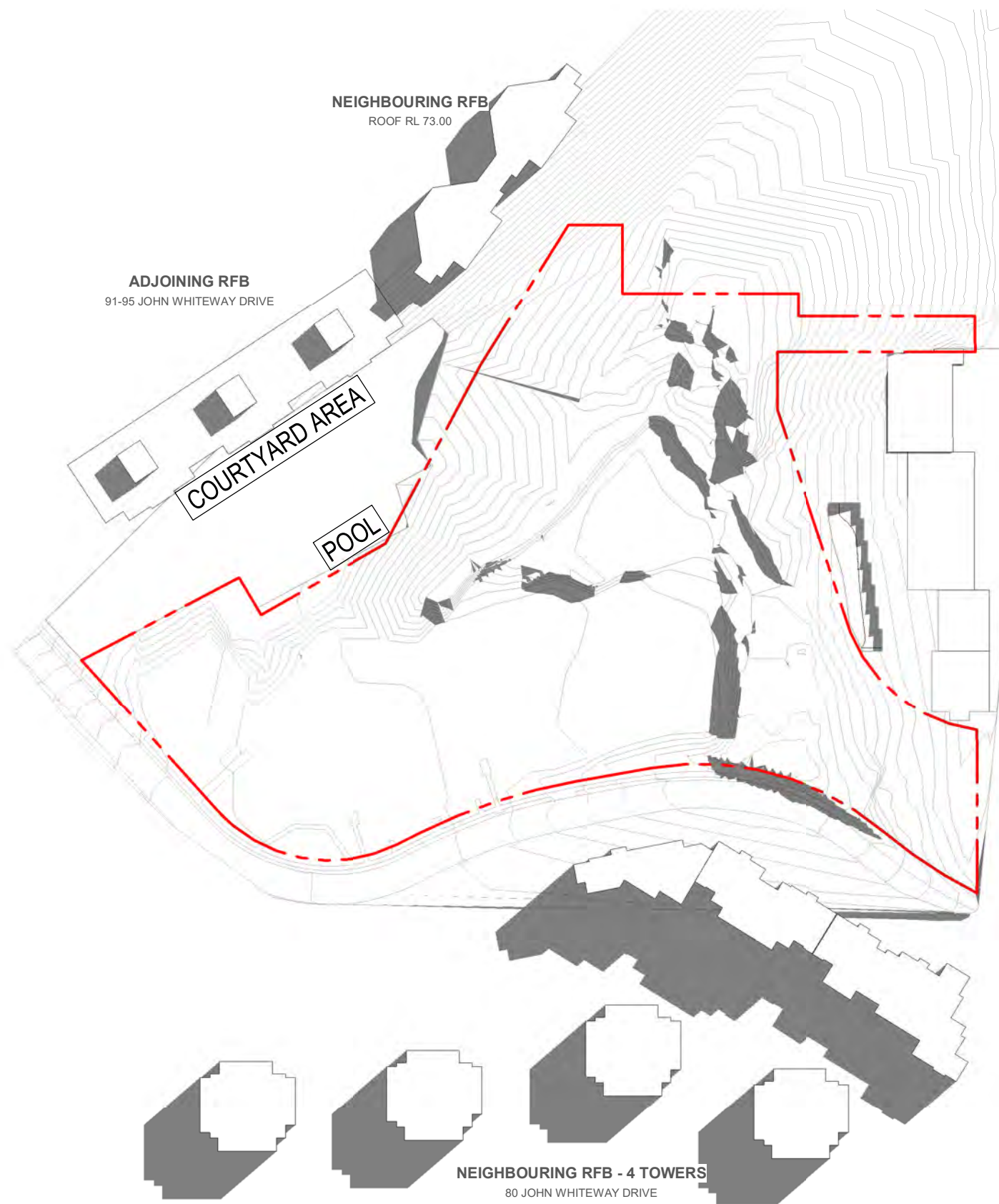
1 IMPACT ON NEIGHBOURING BUILDINGS- 2PM 21 JUNE EXISTING 1: 1500
