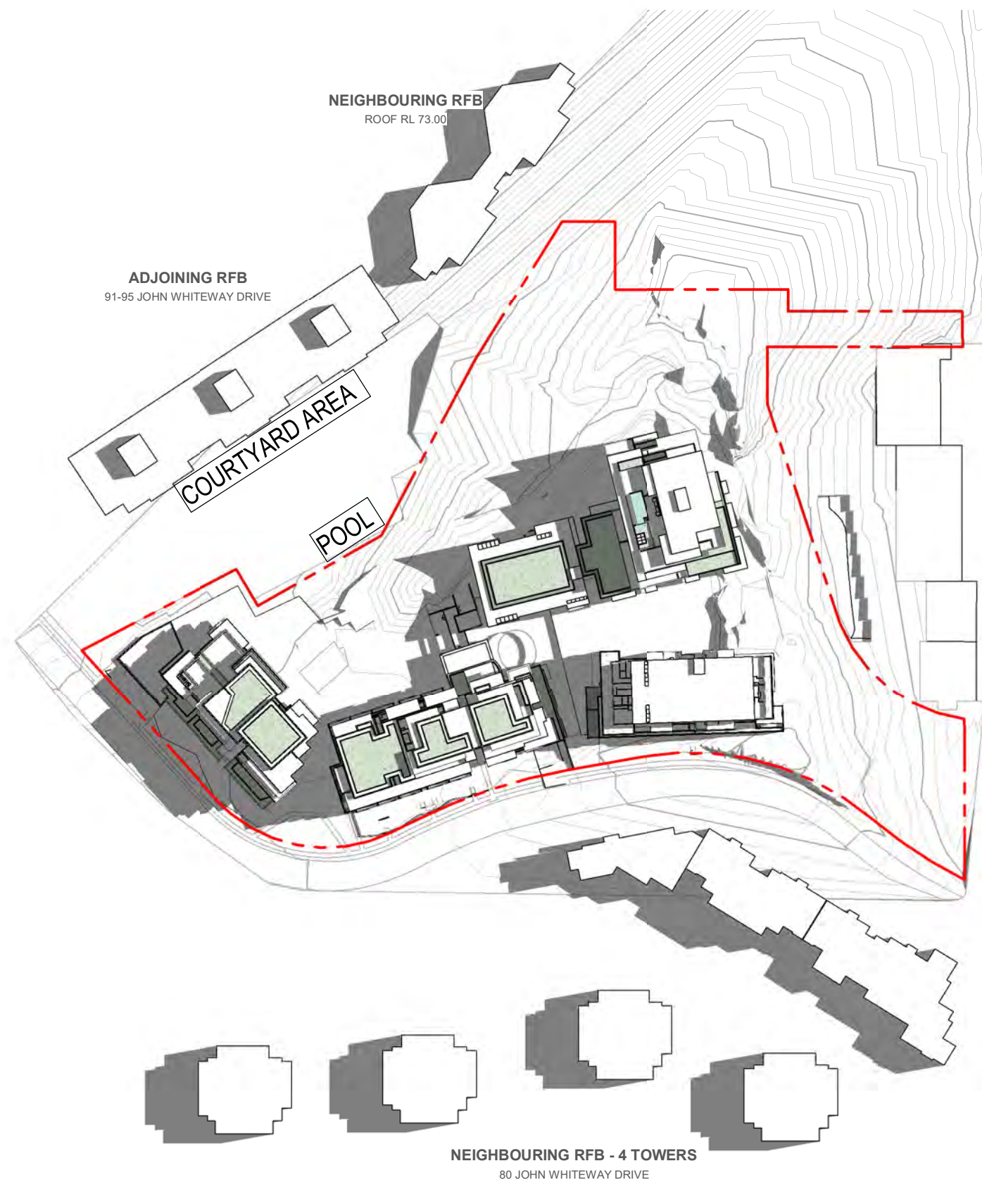
2 IMPACT ON NEIGHBOURING BUILDINGS- 12PM 21 JUNE PROPOSED DA003.1 1 : 1500
