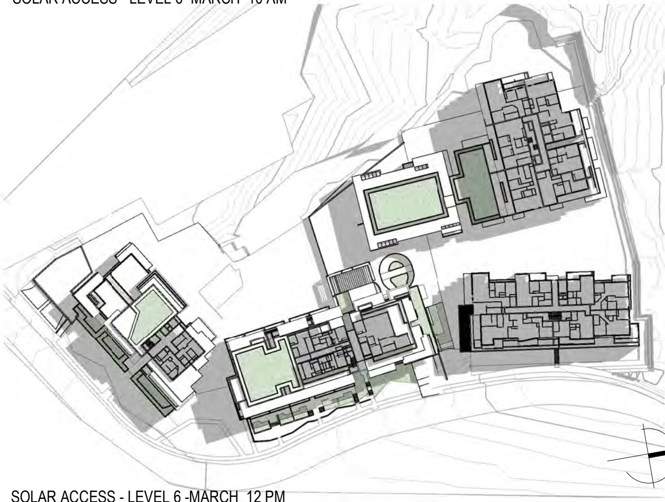
SOLAR ACCESS - LEVEL 6 -MARCH 12 PM
