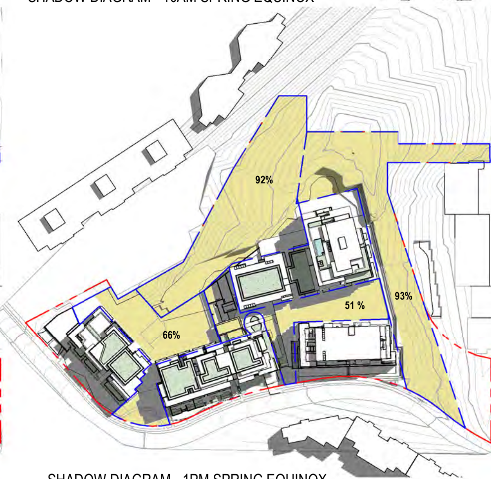
SHADOW DIAGRAM - 1PM SPRING EQUINOX
