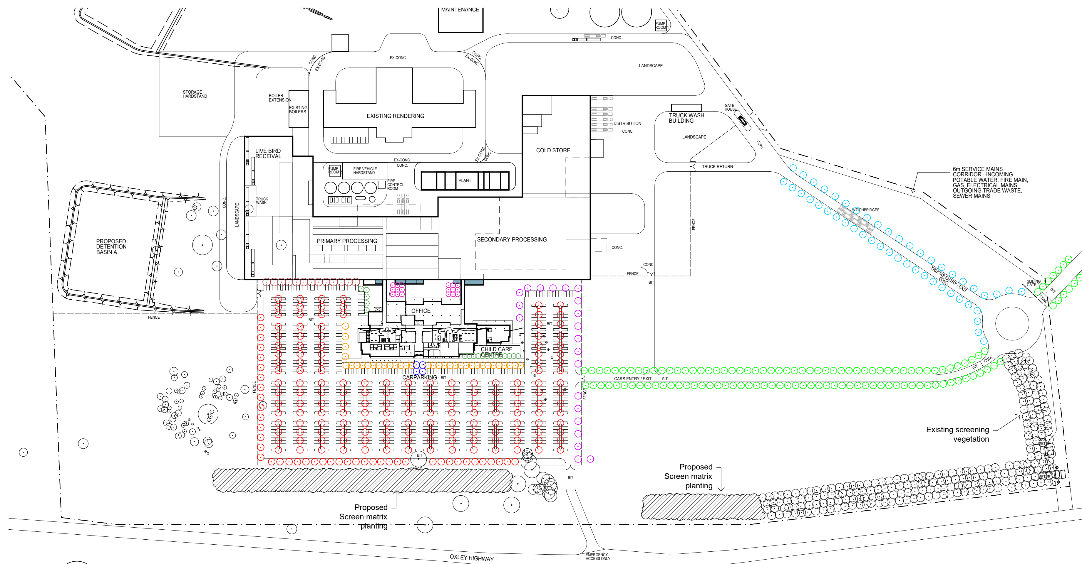
Landscape Tree Plan 1:2000
