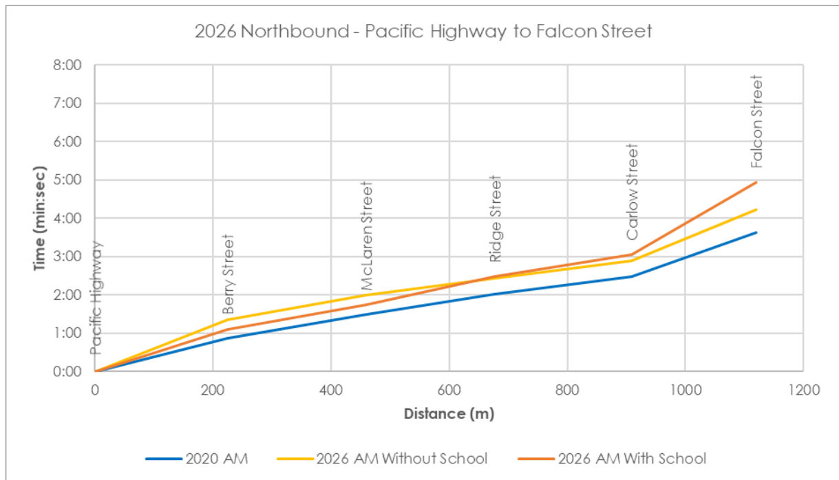
Figure 7.6: 2026 Northbound Travel Time – Morning Peak 8:00am – 9:00am
