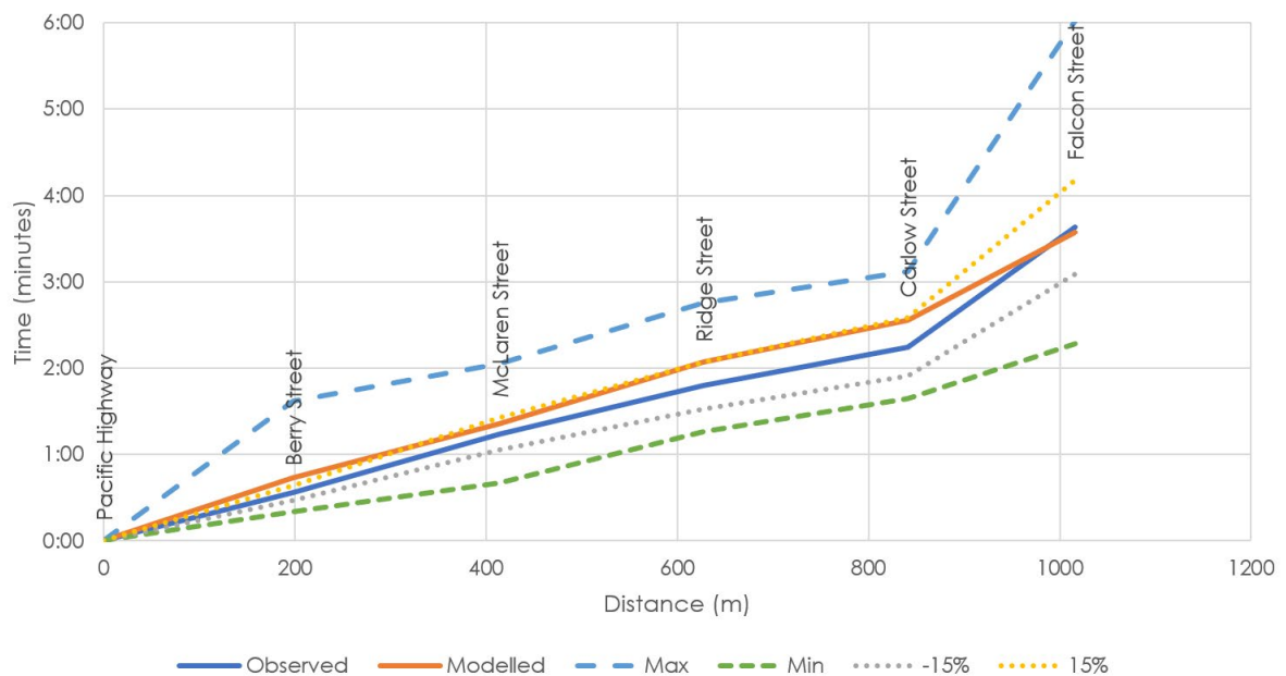
Figure 8.2: Morning Peak Travel Time Northbound (7:45am-8:45am)
