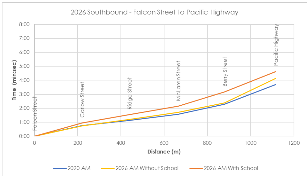
Figure 7.7: 2026 Southbound Travel Time – Morning Peak 8:00am – 9:00am
