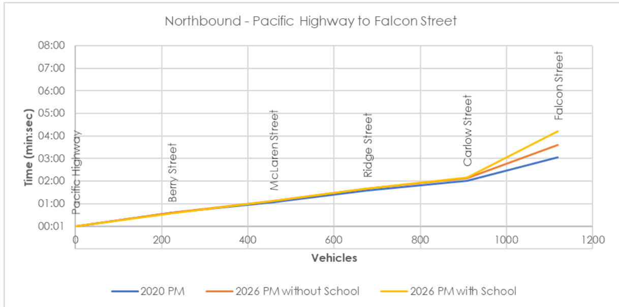
Figure 7.10: 2026 Northbound Travel Time – Evening Peak 3:00pm – 4:00pm
