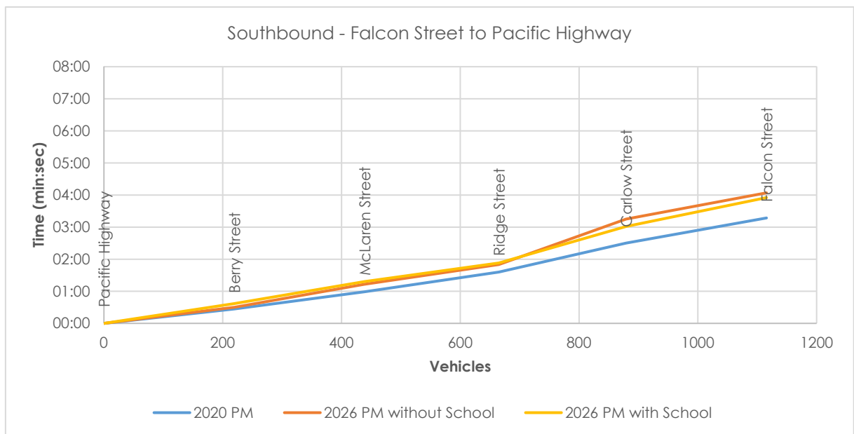
Figure 7.11: 2026 Southbound Travel Time – Evening Peak 3:00pm – 4:00pm
