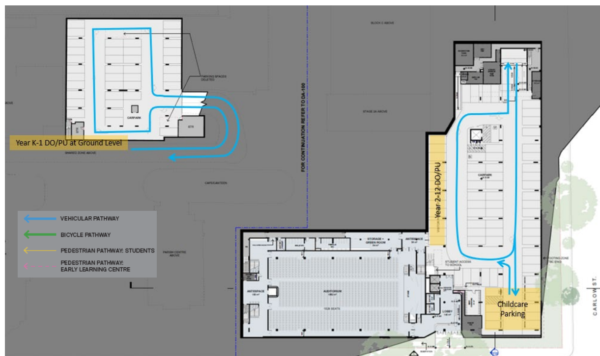
Figure 4.3: Basement Car Park Circulation
