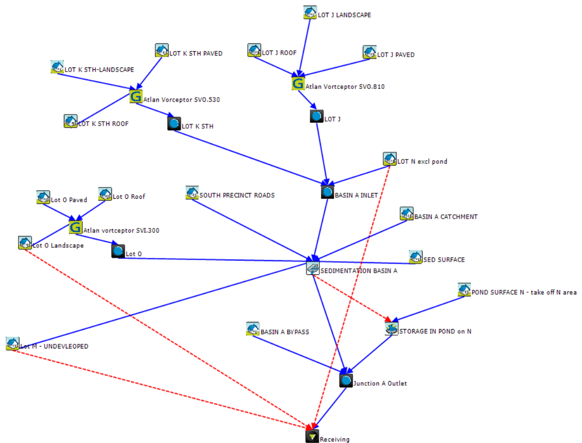
Figure 19 Music Model Southern Catchment – for proposed development stages
