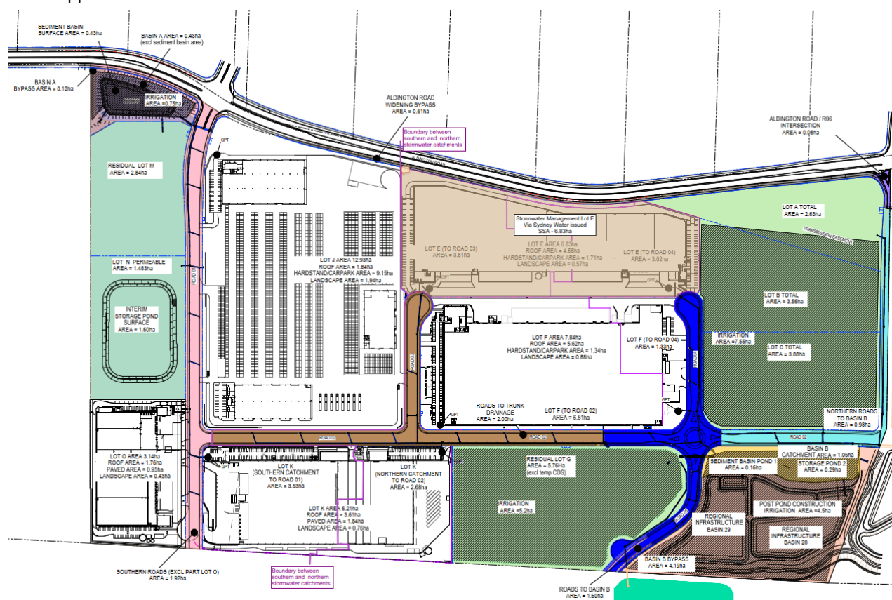
Figure 15 Interim Stormwater management measures – (extract SKC228 for MOD7)
