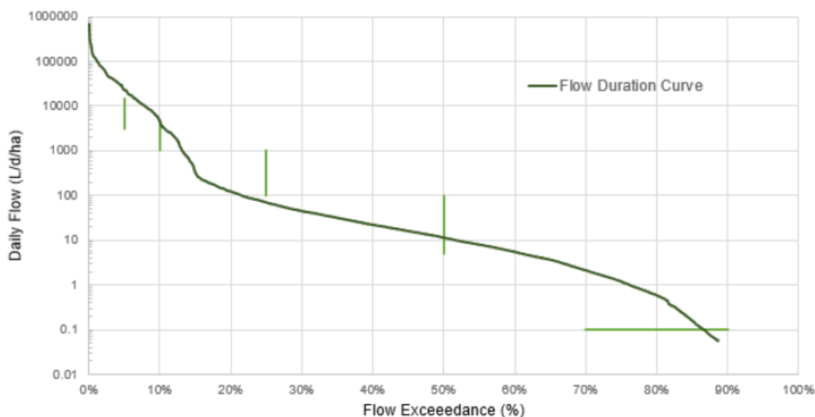
Figure 18: Flow duration curve and targets for proposed development (Northern Catchment)
