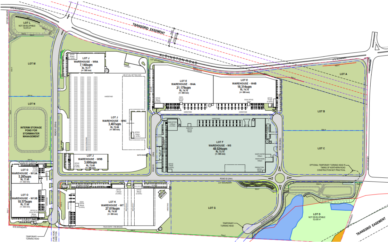
Figure 8: Proposed Lot F, J, K, E and O Development Plan
