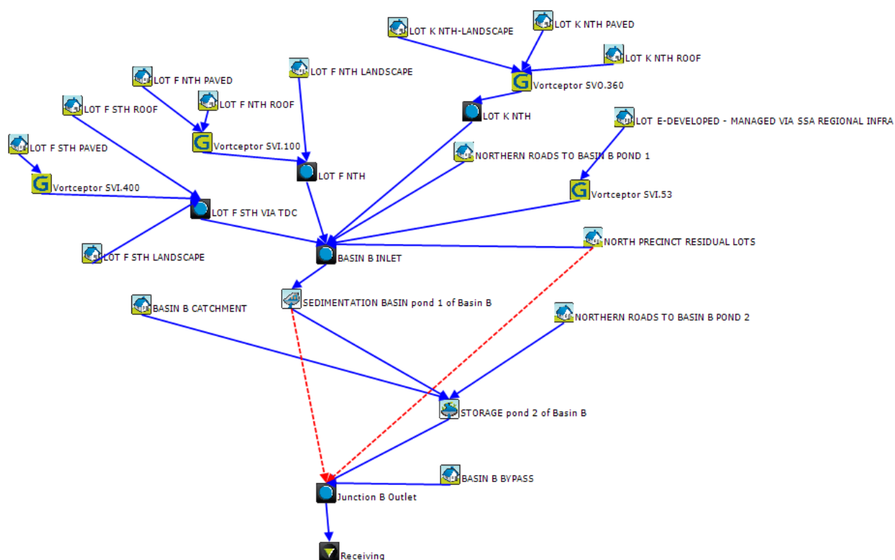
Figure 20 Music Model Northern Catchment – for proposed development
