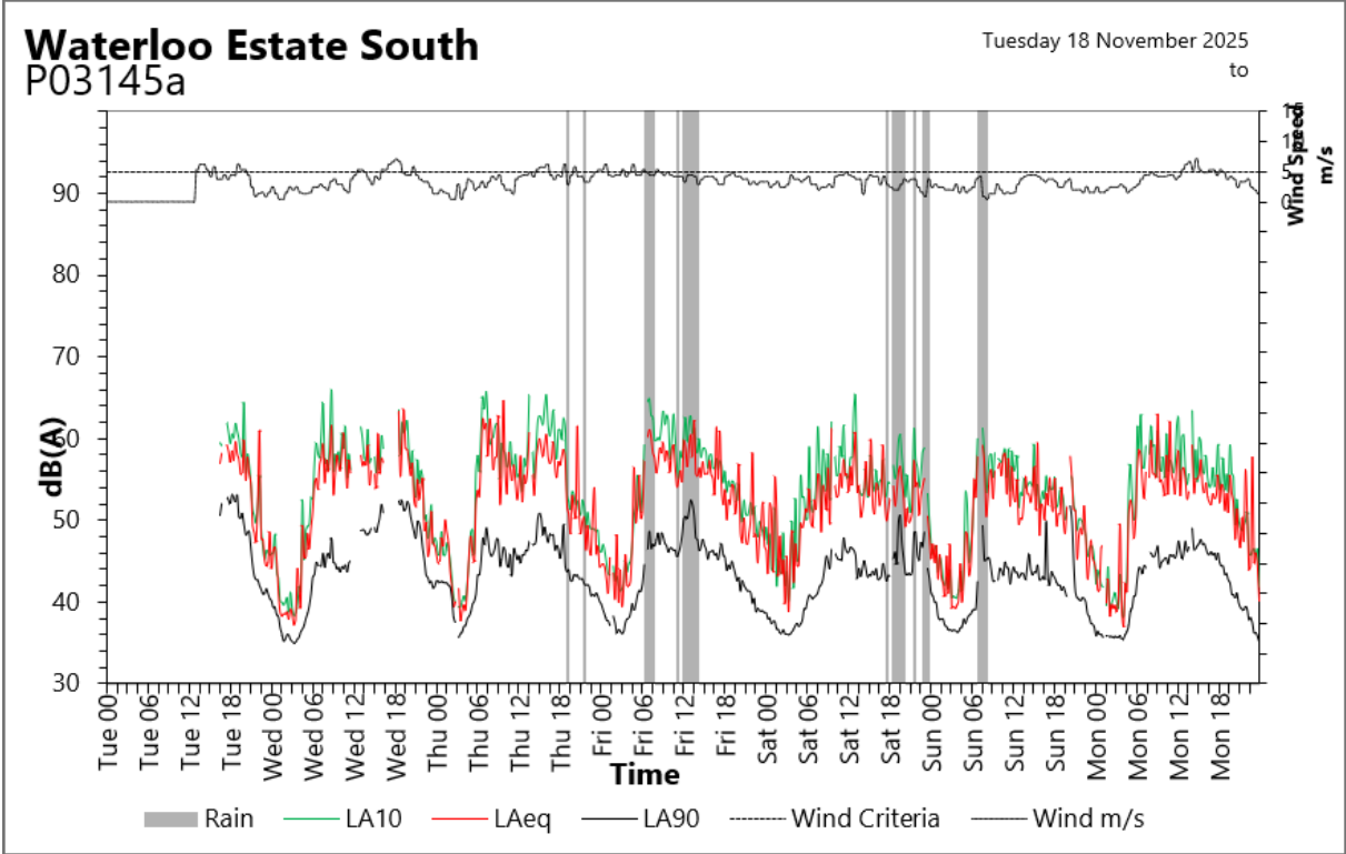
Figure 12: Long-term noise monitoring data graph (LT1)
