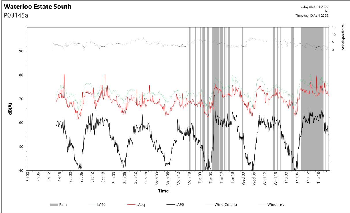
Figure 17: Long-term noise monitoring data graph (LT6)
