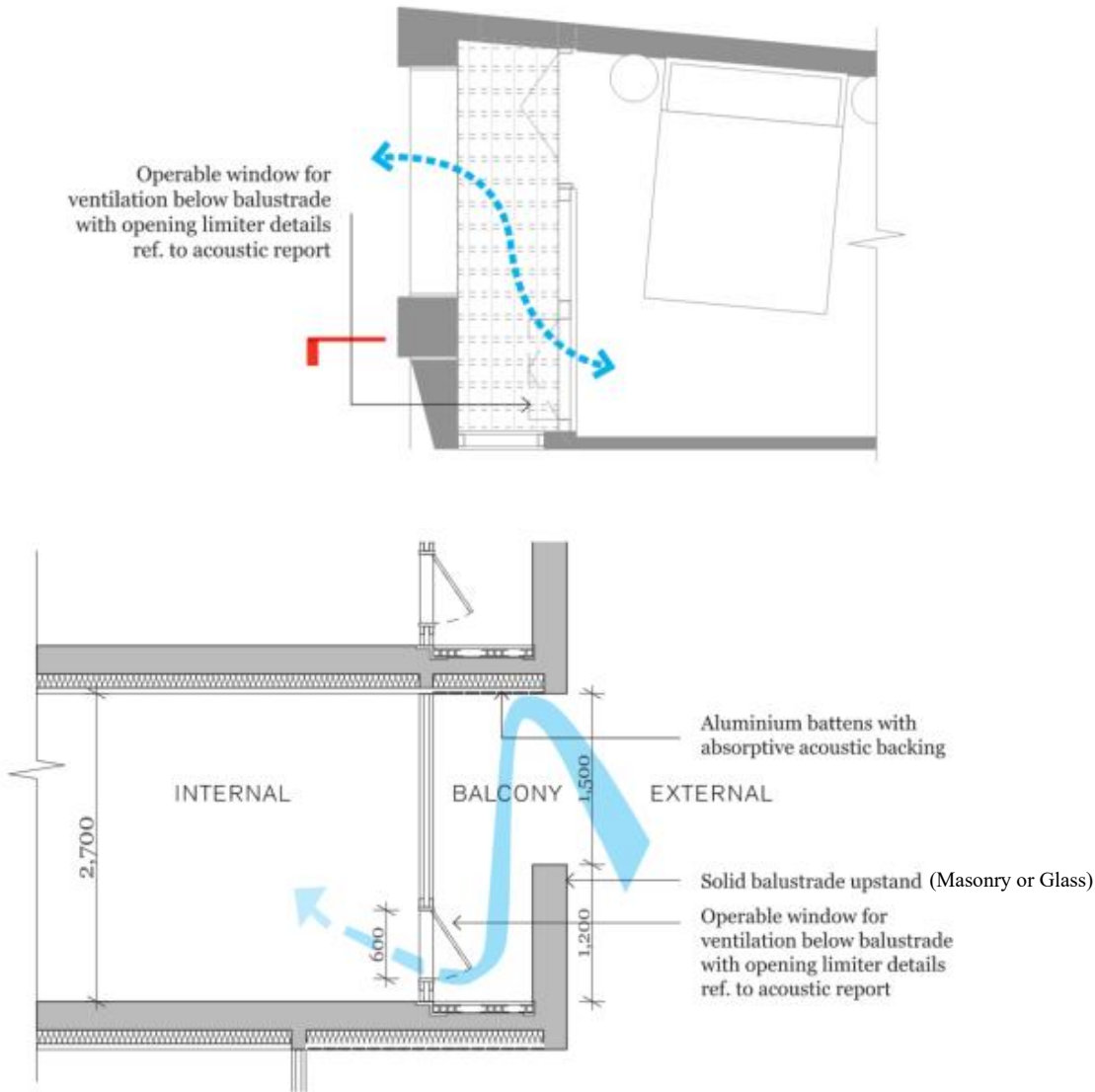
Figure 8: Low level window, treated soffit and solid balustrade upstand (Plan & Section View)
