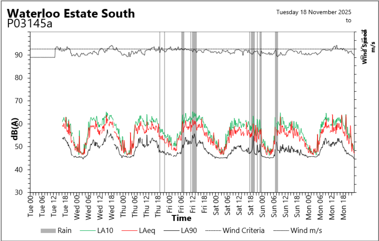
Figure 13: Long-term noise monitoring data graph (LT2)
