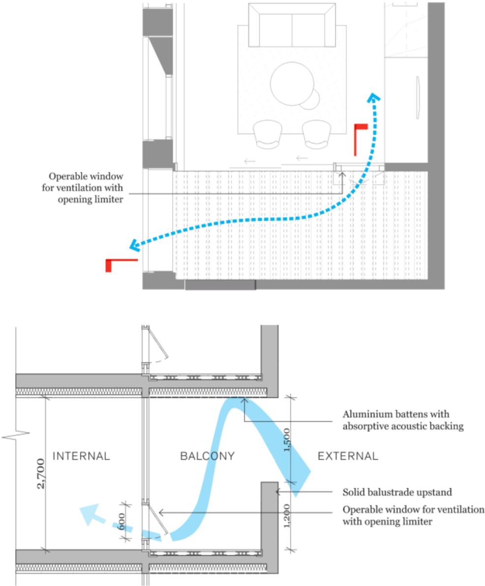
Figure 9: Deep balcony with treated soffit and perpendicular window opening
