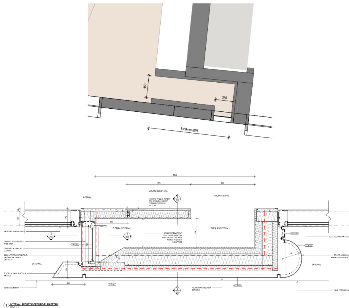
Figure 11: Internal Acoustic Opening (Plan View and Section Detail)
