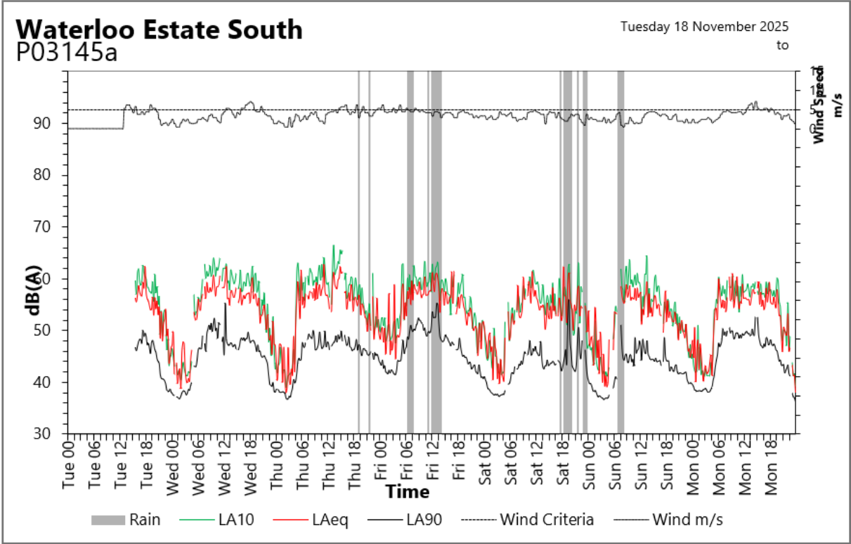
Figure 14: Long-term noise monitoring data graph (LT3)
