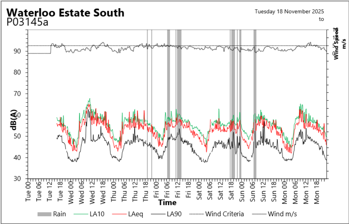
Figure 16: Long-term noise monitoring data graph (LT5)
