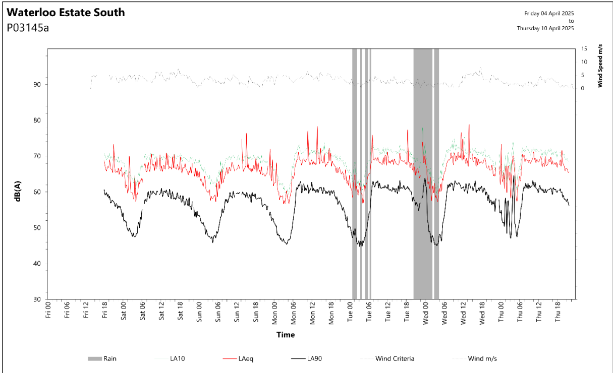
Figure 18: Long-term noise monitoring data graph (LT7)
