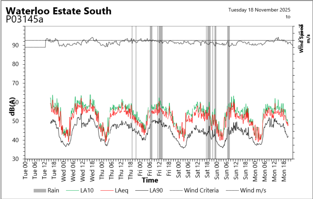
Figure 15: Long-term noise monitoring data graph (LT4)
