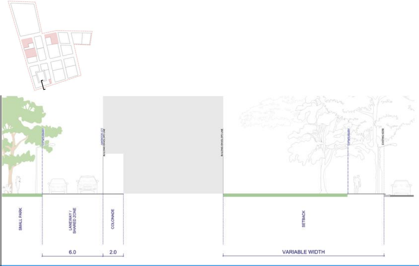
Figure 8(h): STREET CROSS SECTION – Cooper Place
