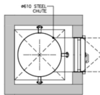
02 SINGLE (610Ø) GALV. STEEL CHUTE LAYOUT
