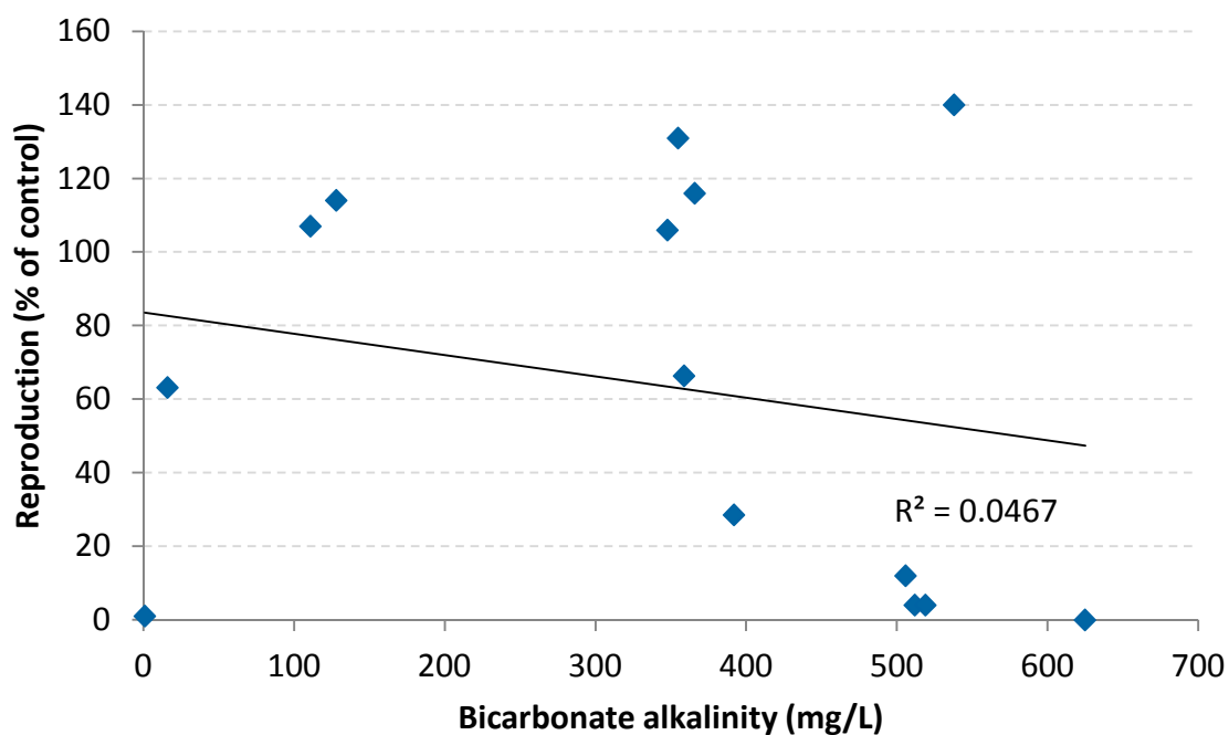
Figure 2-2 Reproduction rates of Cladoceran Compared with Bicarbonate Alkalinity Concentration
