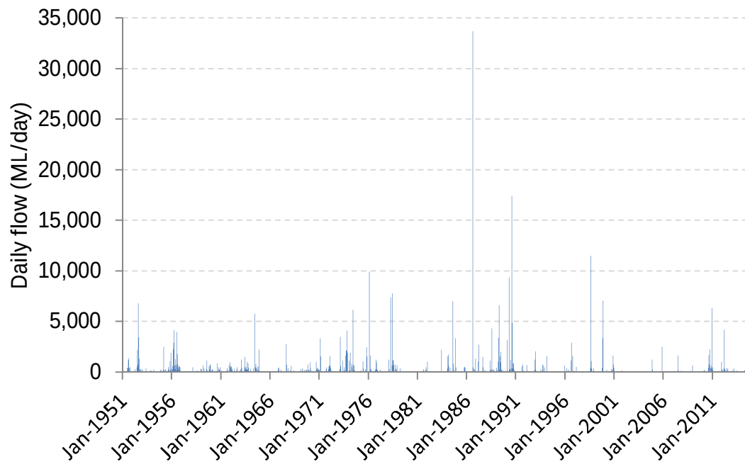
Figure A-3 Observed Flows for Coxs River at Bathurst Road Gauge
