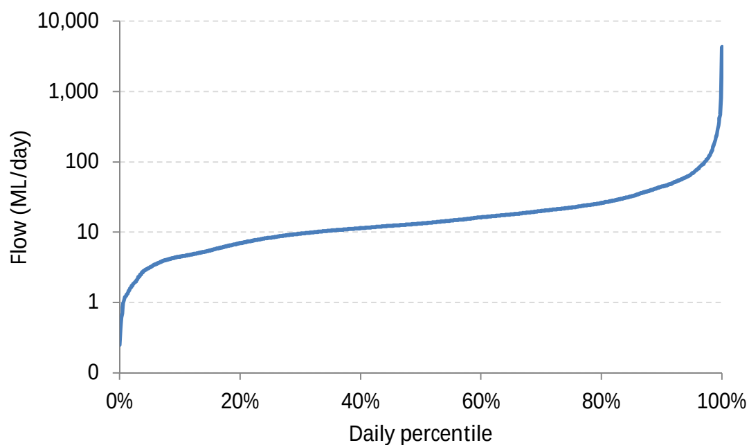
Figure A-2 Daily Flow Percentiles for Coxs River at Wallerawang Power Station Gauge
