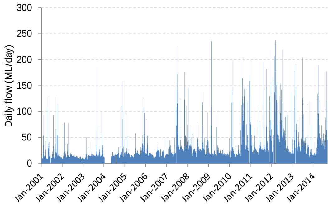
Figure A-5 Observed Flows for Coxs River at Upstream Lake Lyell Gauge
