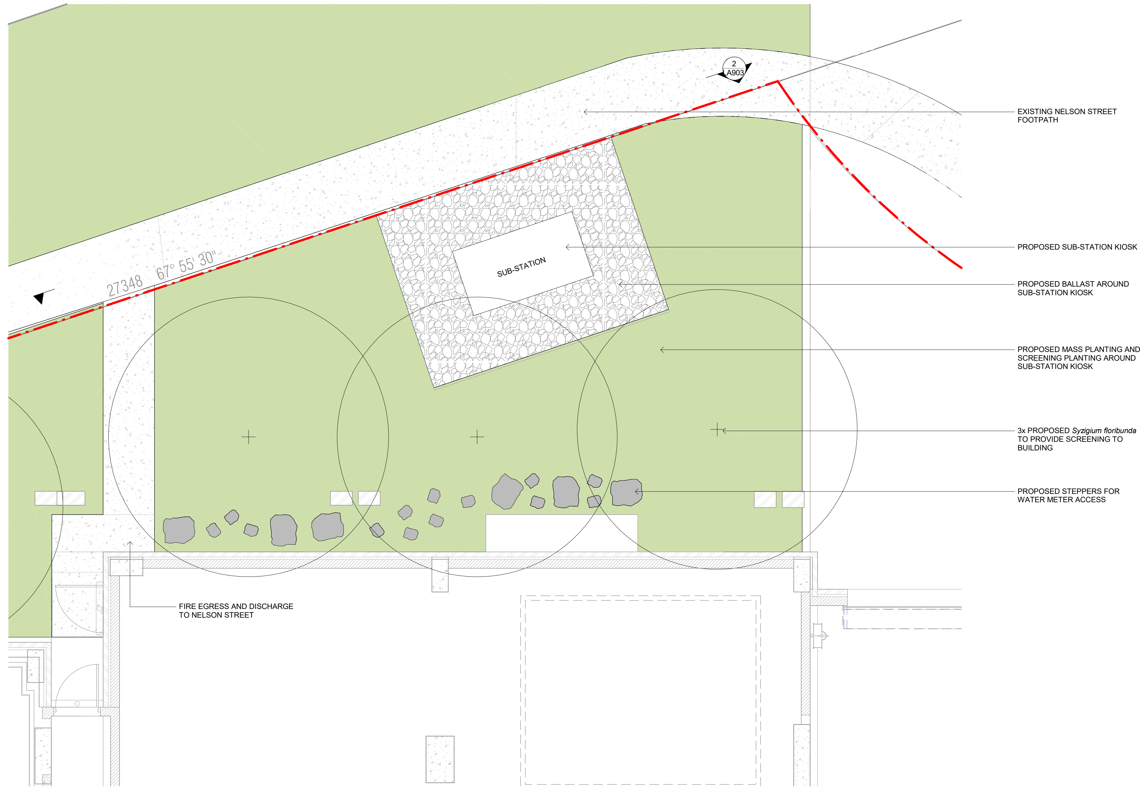
1 DETAILED PLAN - SUBSTATION KIOSK 1:50
