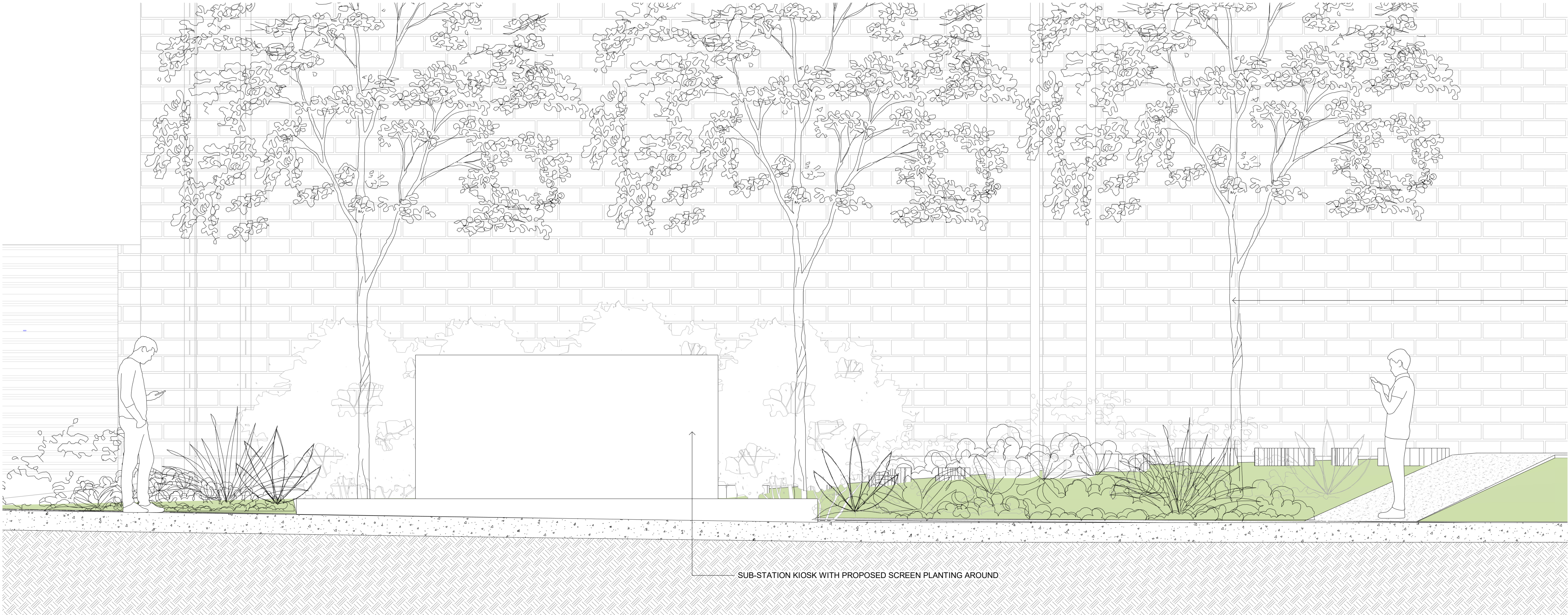
2 DETAILED ELEVATION - SUBSTATION KIOSK INTERFACE TO NELSON STREET LA903 1:25
