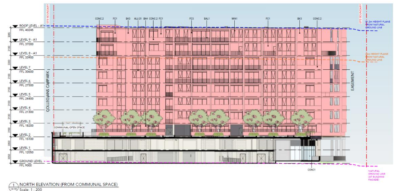
Building 1 – North Elevation
