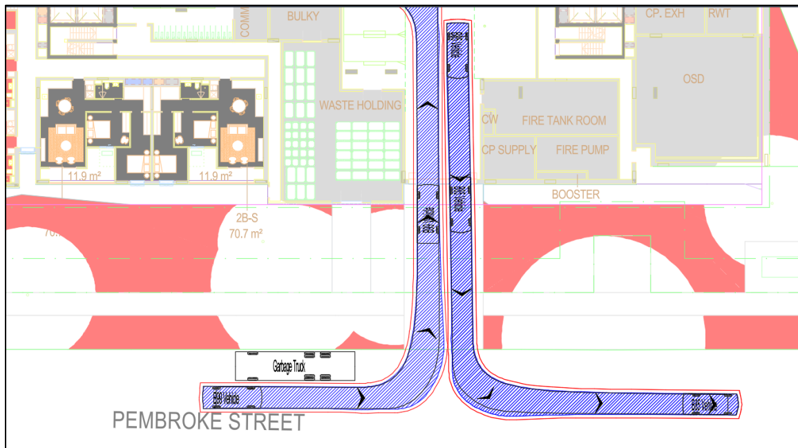
Figure 14 Swept paths analysis – southern building
