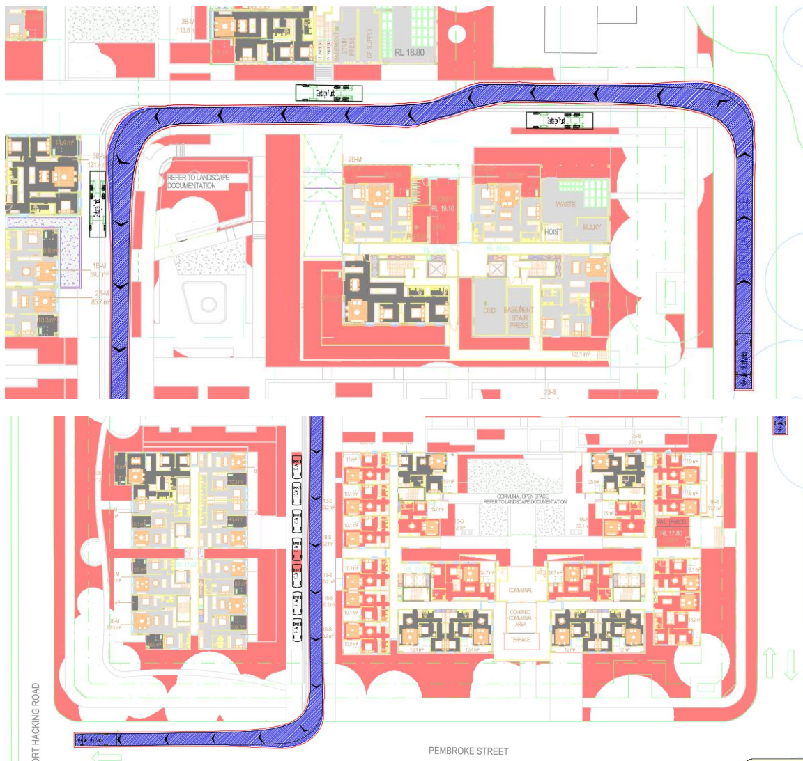
Figure 15 Swept path analysis – internal vehicle circulation
