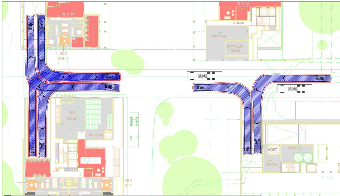
Figure 13 Swept paths analysis – internal roadway
