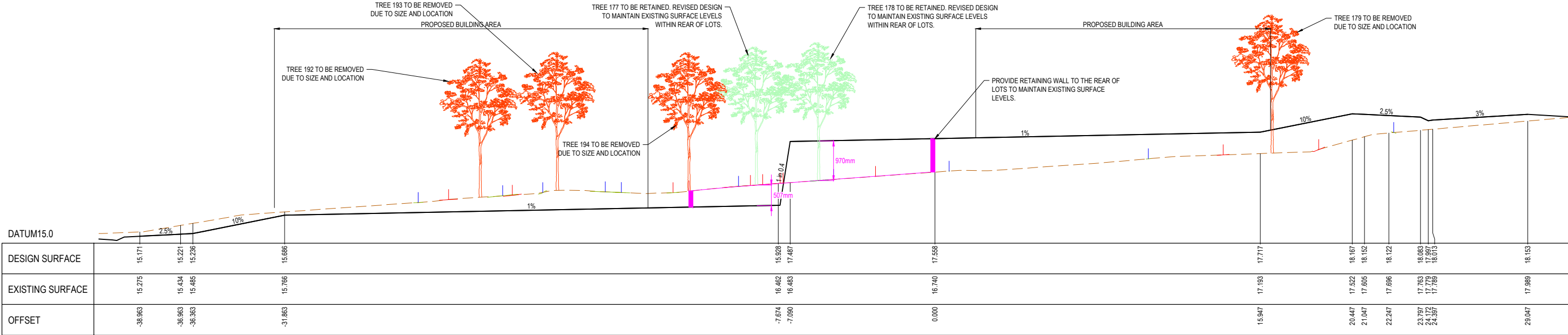
SECTION A TREE 192, 193, 194, 177, 178 & TREE 179
