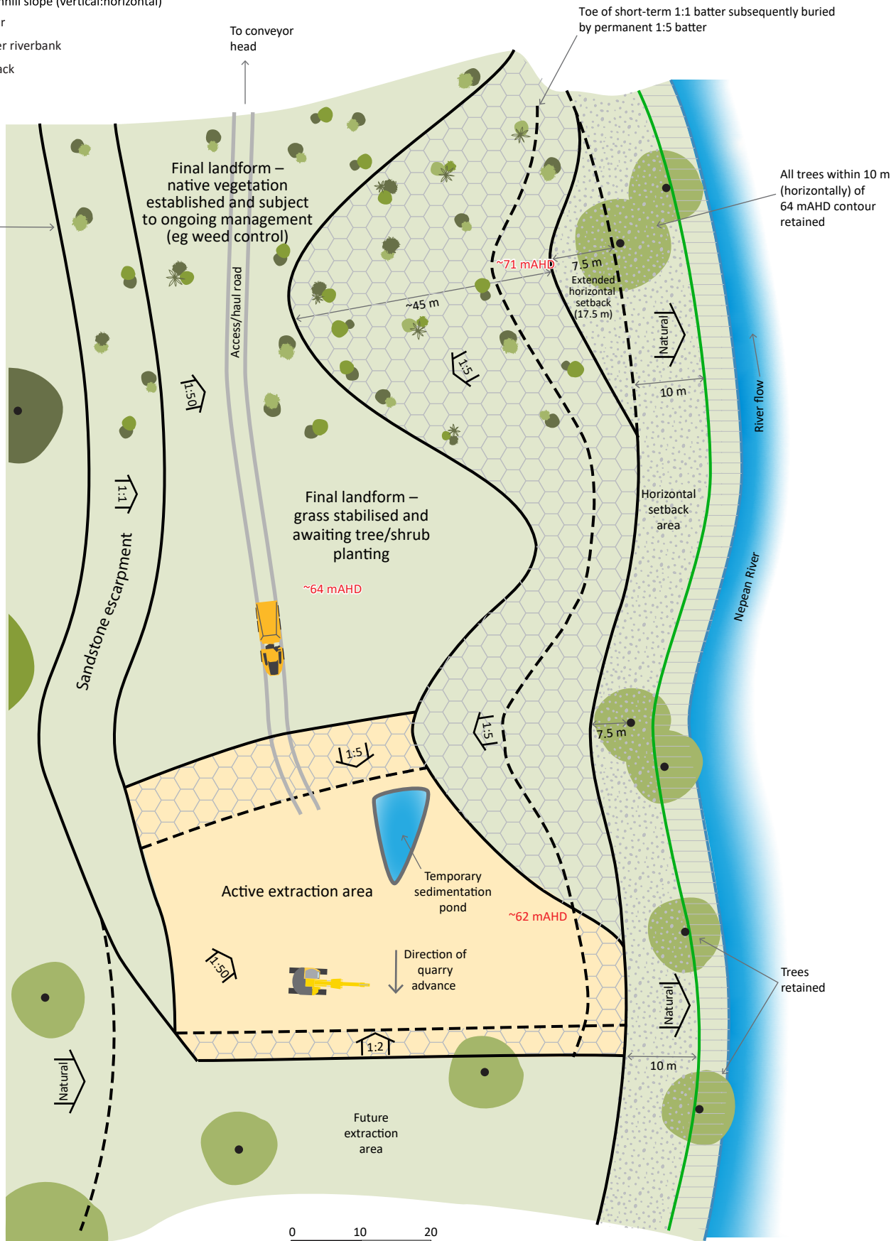
Stage 8 quarrying schematic Menangle Quarry Figure 1.4
