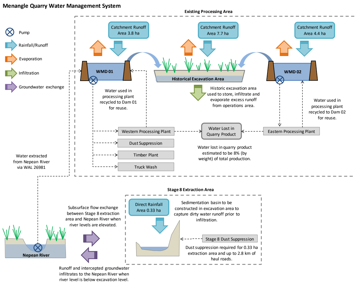
Figure 5.7 Water management system schematic
