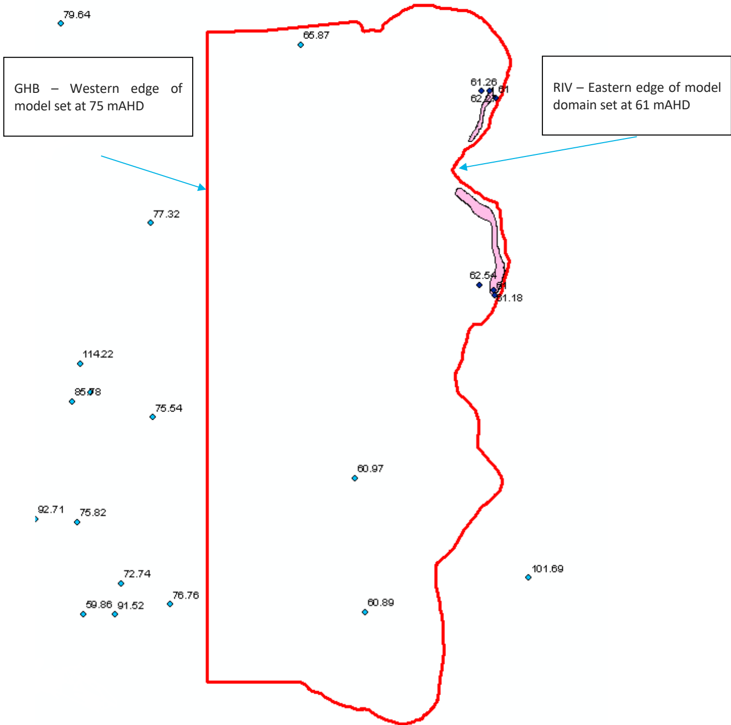
Figure 3.6 Model boundary conditions and regional groundwater levels
