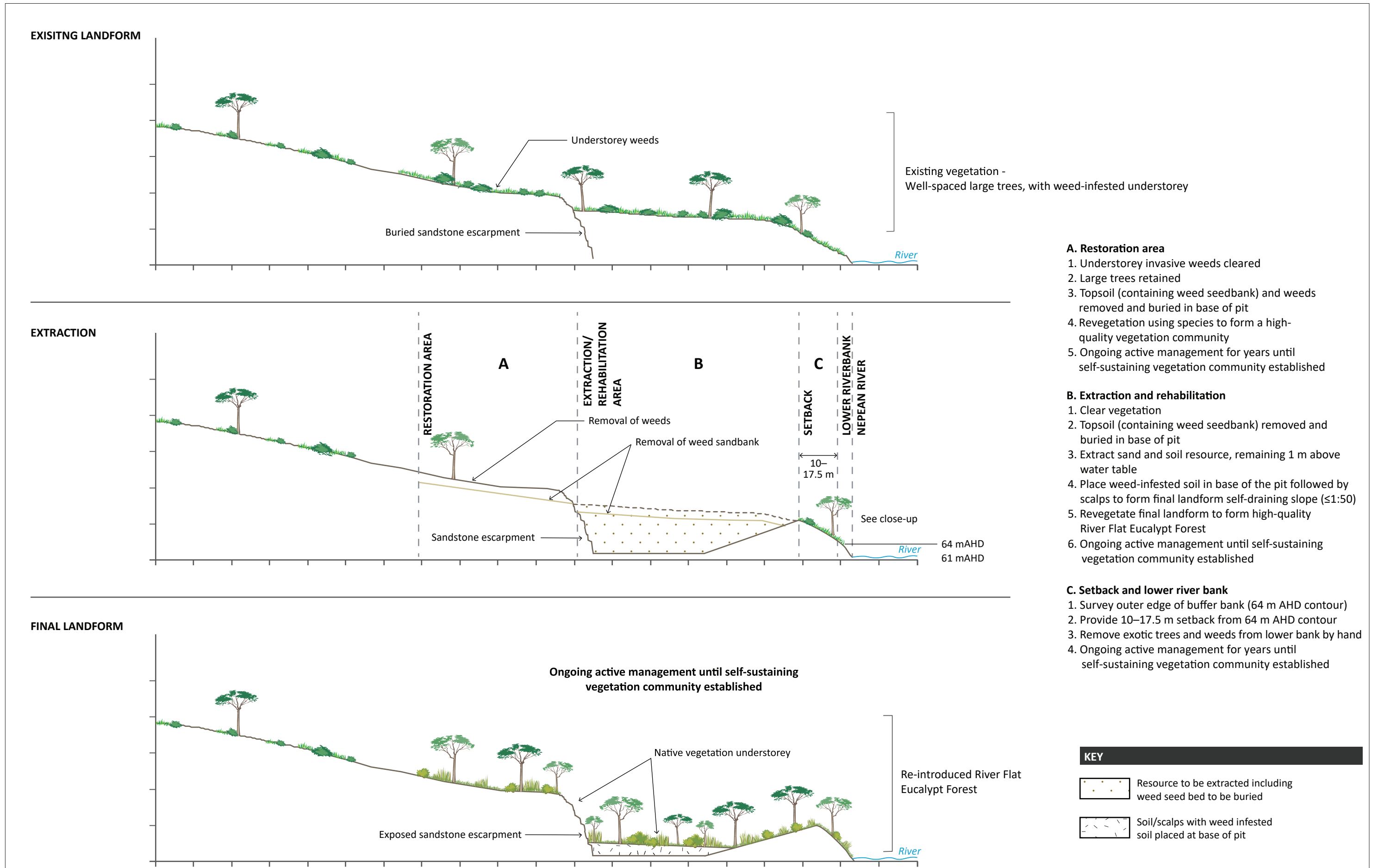
Indicative cross-section Menangle Quarry Extension Figure 5.6
