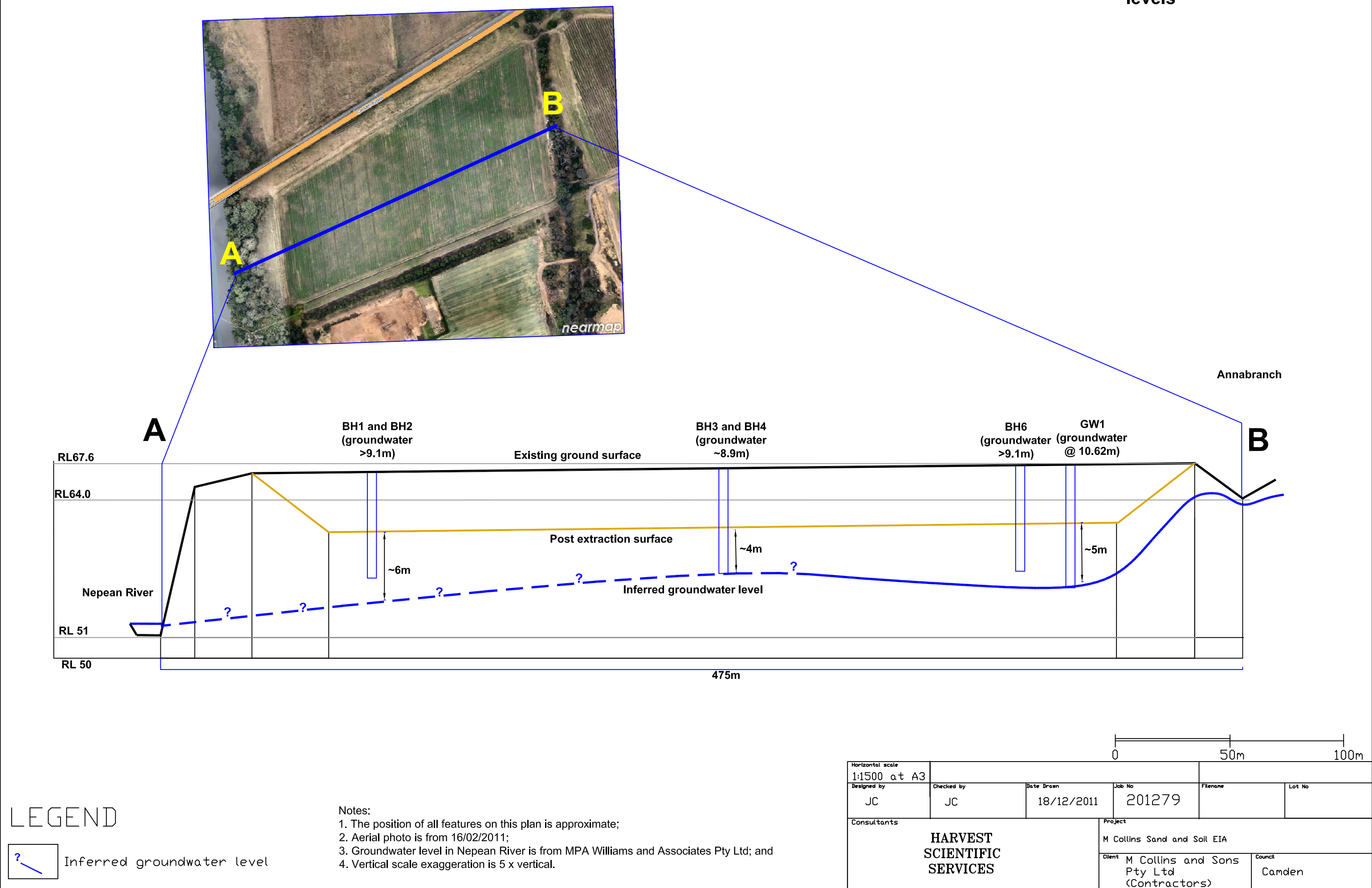
Figure 6 Schematic site long section and inferred groundwater levels
